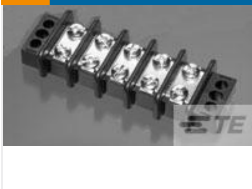
TE 产品编号1546310-8 8P .563" DR BARRIER STRIP
