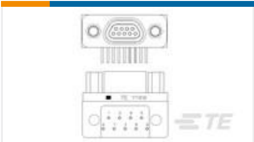
TE 产品编号1532258-3 M83513/13-A01NN = MCKS-N1-B-9SRT1
