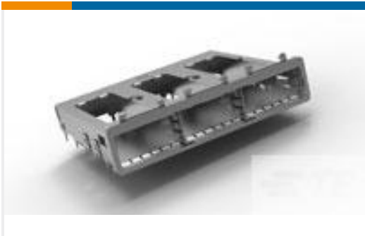
TE 产品编号2007473-1 1x3 QSFP Cage Assy Behind Bzl
