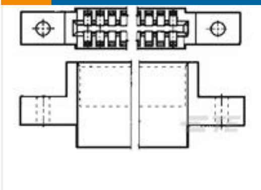
TE 产品编号1-583718-1 TW-LEAF CRP HSG 25 POS 100 C/L
