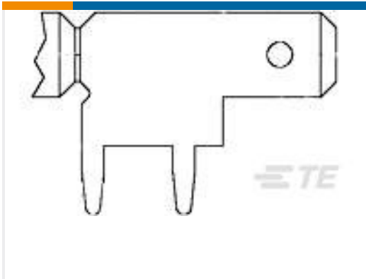
TE 产品编号1217756-1 187 FASTON,TAB,TNBR
