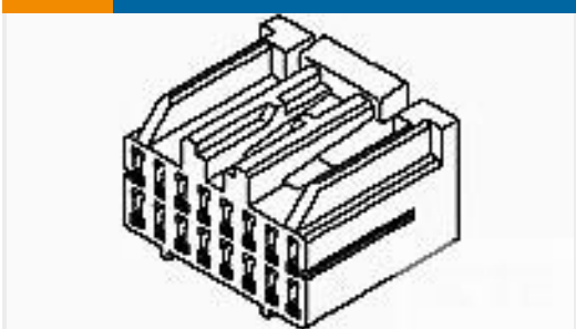
TE 产品编号179678-6 04/07-2 HD HYBRID PLUG ASY 16P
