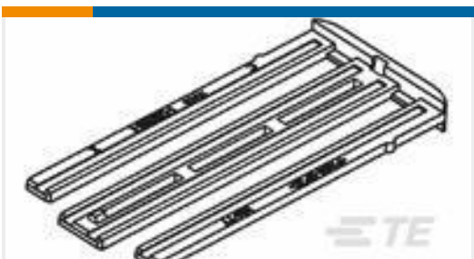
TE 产品编号1-1355118-1 RETAINER FOR 60POS SOCKET HSG
