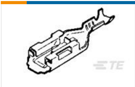
TE 产品编号170454-1 PL 250 AUTOMOTIVE REC 18-14 0.40 X 21 BR
