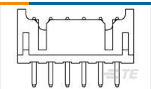
TE 产品编号1470109-6 2.0mm Pitch Header,Dip 6p
