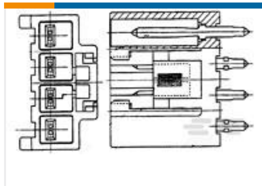
TE 产品编号1-178487-1 UP 3.96 4P TAB HDR NAT TYPE 2
