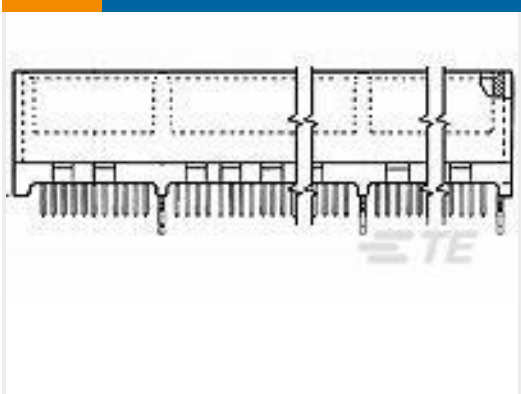
TE 产品编号1-5145168-2 STANDARD EDGE .050 SERIES 92 DUAL ASSY
