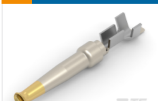
TE 产品编号1-66504-0 D-Sub Conn Contacts: Socket, Phosphor Bronze, Signal, Size 20
