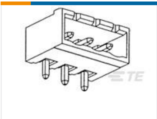
TE 产品编号1546109-4 EUROSTYLE TB,HEADER,GREY,4 POS
