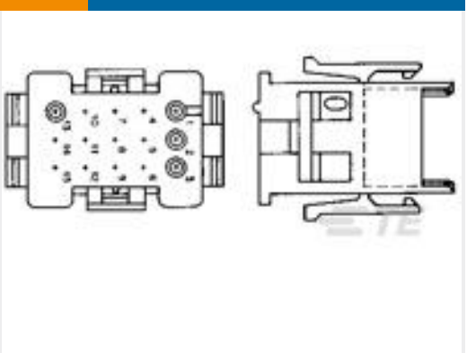
TE 产品编号1-640511-0 09P MR II CAP HSG V0 RED
