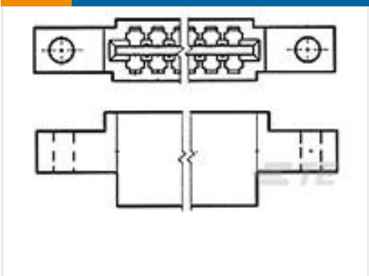
TE 产品编号480110-2 HSG AMP LEAF 15 POS
