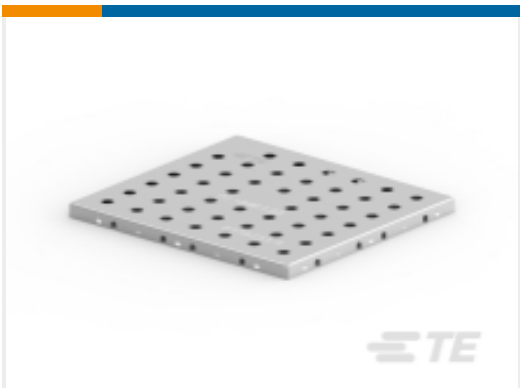
TE 产品编号2118723-4 STD SHIELD COVER, AL-37.33X34.18X2.00MM
