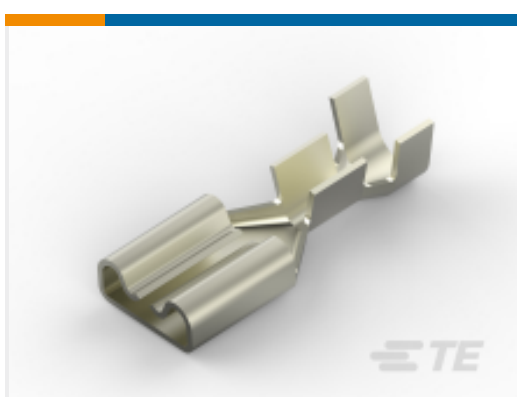
TE 产品编号2238143-1 250 FASTON,REC.,22-18 AWG,NPST
