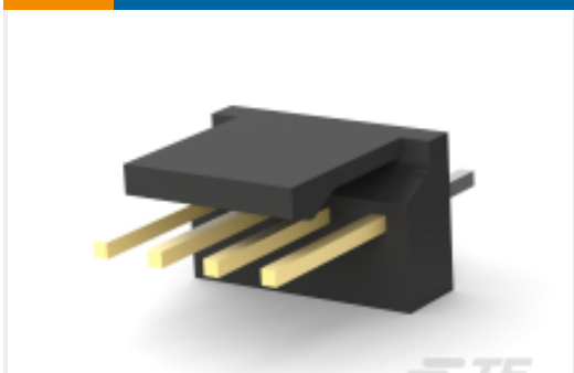
TE 产品编号3-647116-2 Nylong Vertical PCB Header: 2.54mm, Through Hole, MTA 100
