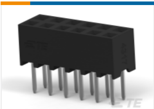
TE 产品编号1-2314820-2 12P,2MM,B-B,REC,DRV,T,2.7,0.1AU,TB
