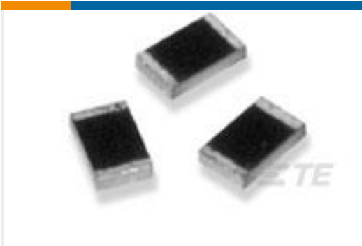
TE 产品编号1-1879263-9 RP 2B 33K2 0.1% 15PPM CUT LENGTH
