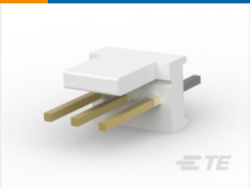
TE 产品编号1-640454-2 Polyester Vertical PCB Header: 2.54 mm, With Mating Alignment, Unshrouded
