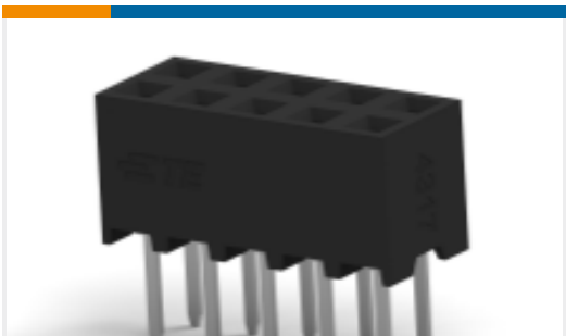
TE 产品编号1-2314820-0 10P, 2MM, B-B, REC, DRVT, 2.7, 0.1AU, TB
