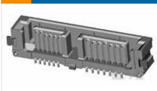
TE 产品编号1735574-3 Assembly Slimline SATA Plug Vertical, TH
