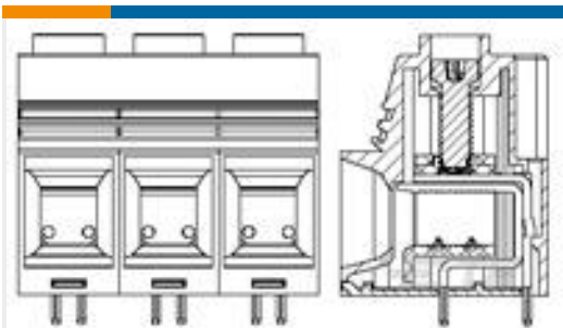
TE 产品编号1986242-3 Power Connector, 15.0mm, Green, 3 posn
