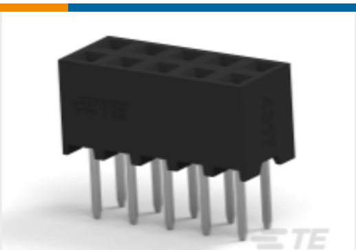
TE 产品编号1-2314820-0 10P,2MM,B-B,REC,DRV T,2.7,0.1AU,TB
