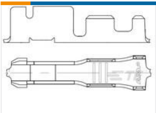
TE 产品编号2178453-1 .090 CLUSTER REC.
