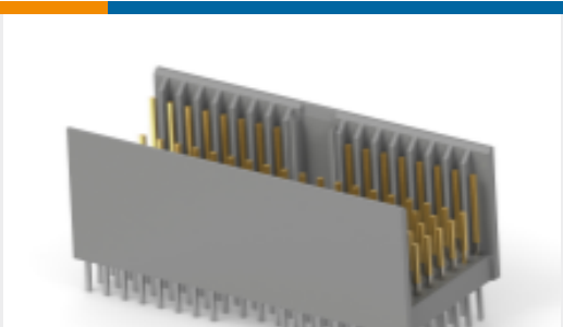
TE 产品编号5646530-1 Z-PACK 2MM HM TYPE A/B 127P
