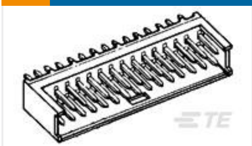
TE 产品编号280385-3 2X8P AMPMODU II SHRD HDR,ST,0.76 AU
