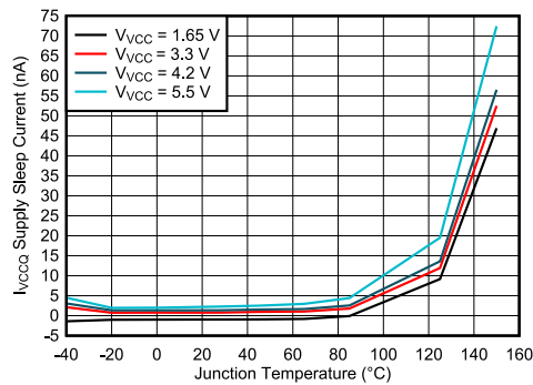
Figure 7-4. Sleep Current ( I_{VCCQ} ) vs. Junction Temperature ( T_J )
