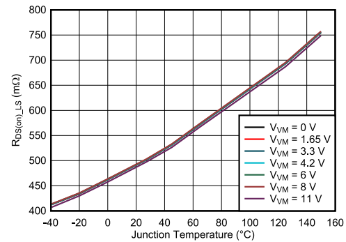
Figure 7-12. High-Side R_{DS(on)} vs. Junction Temperature ( T_J )
