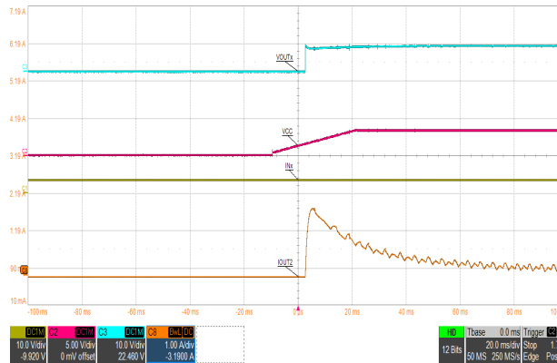
A. Channel 1 = IN1, Channel 2 = V CC Channel 3 = V OUT IN2 (paralleled) (OUT1/2 paralleled) Channel 8 = Motor Current
