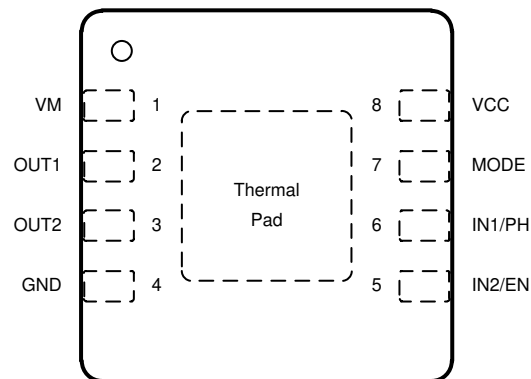
Figure 6-2. DRV8210 DSG Package 8-Pin WSON Top View
