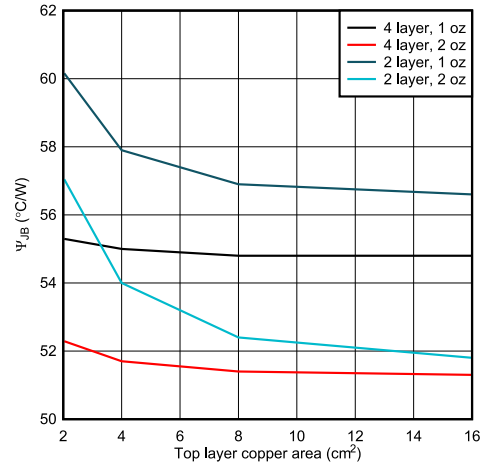
Figure 9-31. WSON, junction-to-board characterization parameter vs copper area
