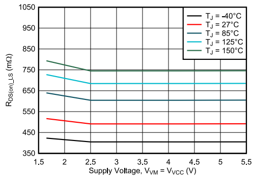
Figure 7-13. Low-Side R_{DS(on)} vs. Supply Voltage
