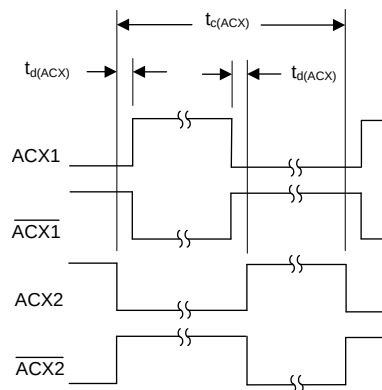
图 7. AC-Excitation Timing Characteristics
