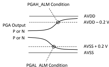
图 13. PGA Monitor Thresholds
