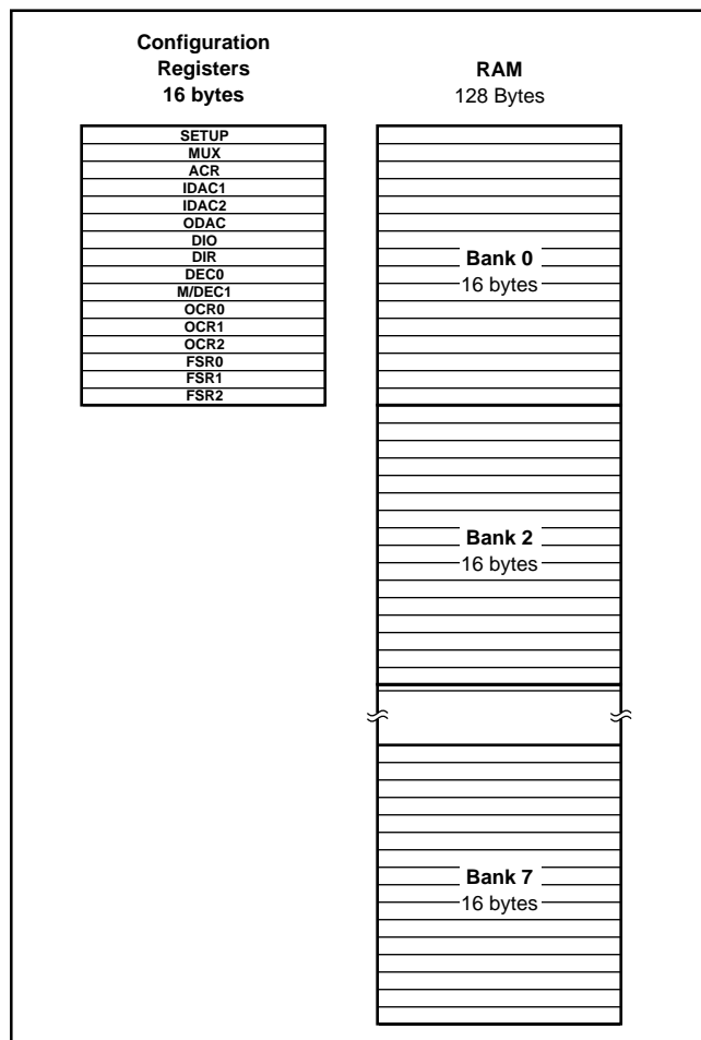
FIGURE 5. Memory Organization.
