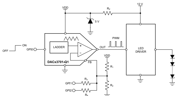
Automotive Brake Light With the DACx3701-Q1
