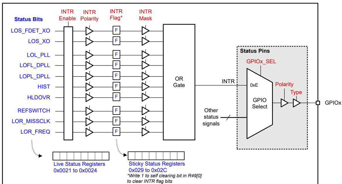
Figure 9-22. Status and Interrupt
