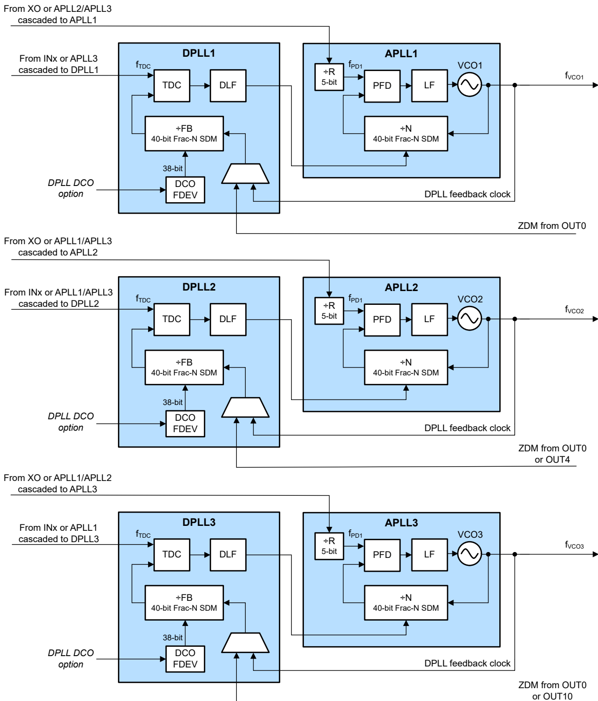
Figure 9-2. PLL Architecture
