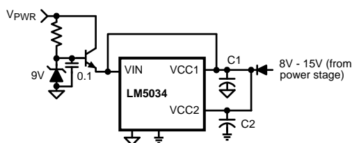
Figure 27. Start-up Regulator for V_{PWR} >100V
