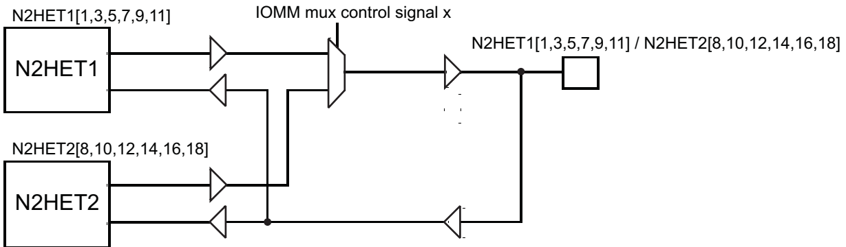
Figure 7-18. N2HET Monitoring
