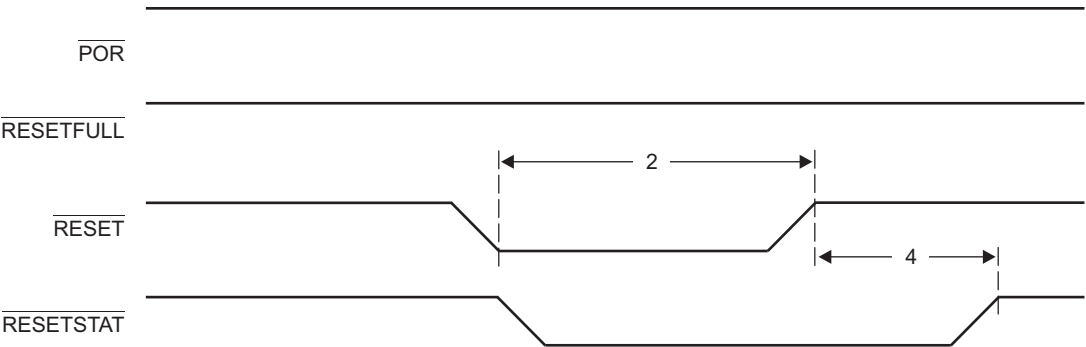
Figure 7-5 Soft/Hard-Reset Timing
