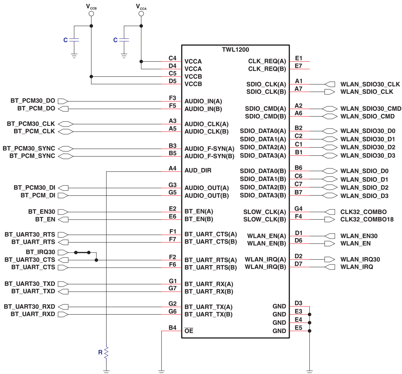
Figure 25. Application Circuit Example, \overline{\text{OE}} Connection With Audio_CLK and Audio_F-SYNC Channels Established From B Side to A Side
