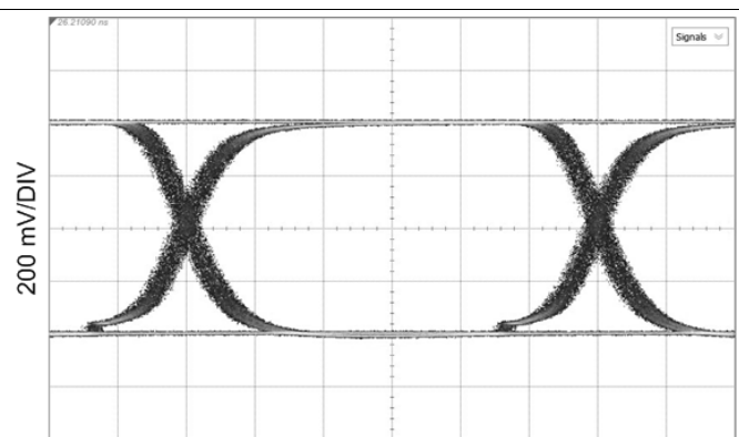
CD Mode, measured at SDI_IO+ HOST_EQ0 = F, SDI_OUT_SEL = H, OUT_CTRL = F Figure 29. 270 Mbps, TL = 20" FR4, Reclocked
