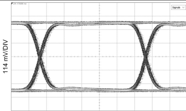
EQ Mode, measured at OUT0± HOST_EQ0 = F, SDI_OUT_SEL = H, OUT_CTRL = F Figure 24. 2.97 Gbps, CC = 200-m Belden 1694A, Reclocked
