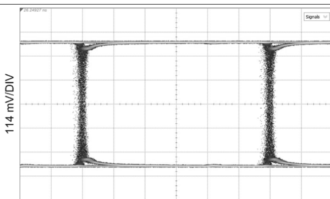
EQ Mode, measured at OUT0± HOST_EQ0 = F, SDI_OUT_SEL = H, OUT_CTRL = F Figure 28. 270 Mbps, CC = 600-m Belden 1694A, Reclocked
