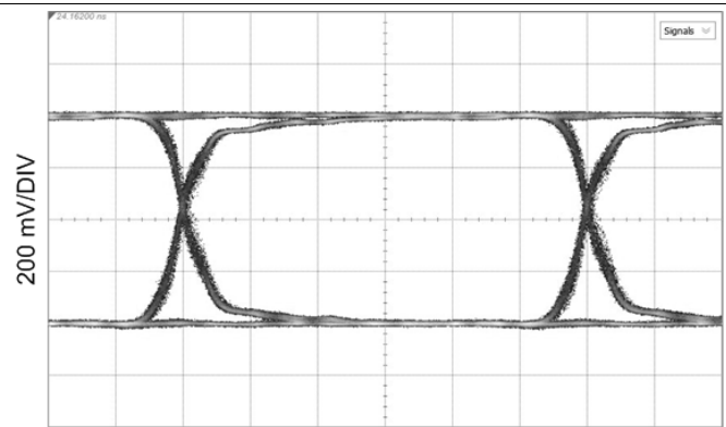
CD Mode, measured at SDI_IO+ HOST_EQ0 = F, SDI_OUT_SEL = H, OUT_CTRL = F Figure 27. 1.485 Gbps, TL = 20" FR4, Reclocked
