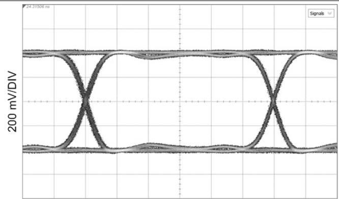
CD Mode, measured at SDI_IO+ HOST_EQ0 = F, SDI_OUT_SEL = H, OUT_CTRL = F Figure 25. 2.97 Gbps, TL = 20" FR4, Reclocked
