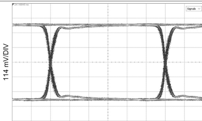
EQ Mode, measured at OUT0± HOST_EQ0 = F, SDI_OUT_SEL = H, OUT_CTRL = F Figure 26. 1.485 Gbps, CC = 300-m Belden 1694A, Reclocked
