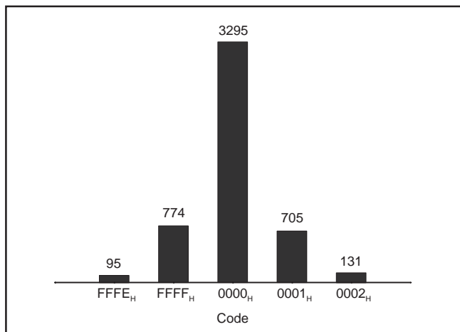
FIGURE 12. Histogram of 5000 Conversions of a DC Input at the Code Transition, 5V Operation External Clock Mode.
