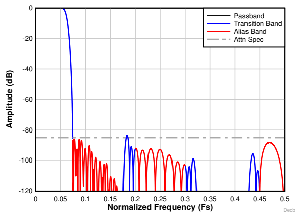
图 8-28. Decimation by 8 complex frequency response
