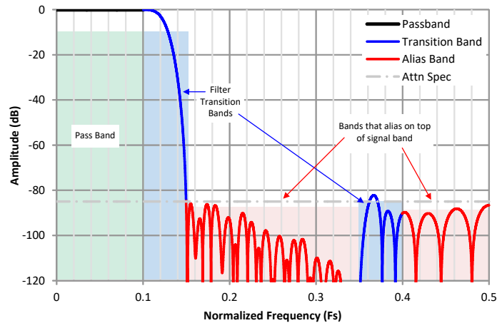
图 8-23. Interpretation of the Decimation Filter Plots
