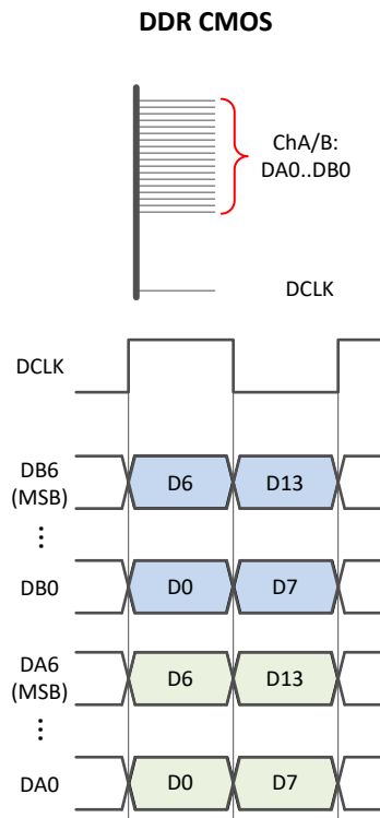
图 8-35. Output Data Format in Real Decimation
