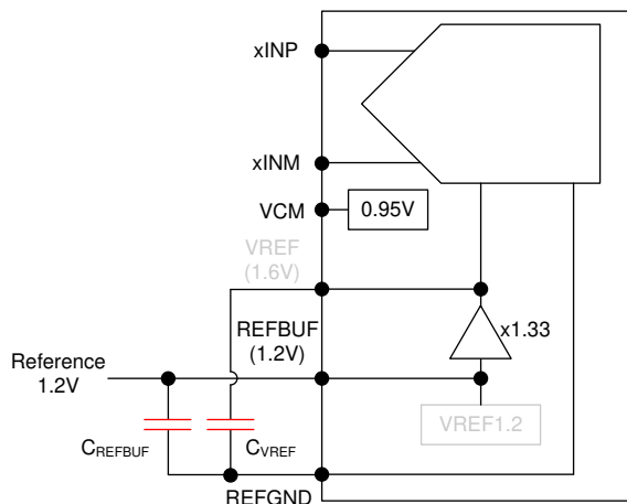
图 8-17. External 1.2V reference using internal reference buffer
