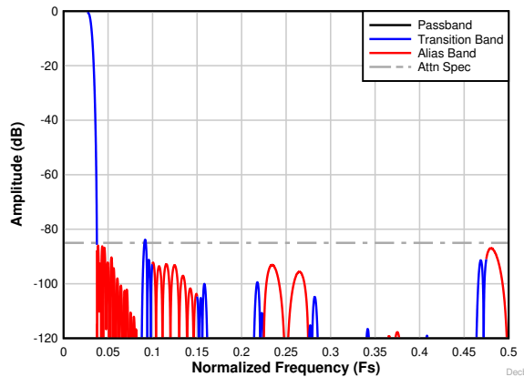
图 8-30. Decimation by 16 complex frequency response
