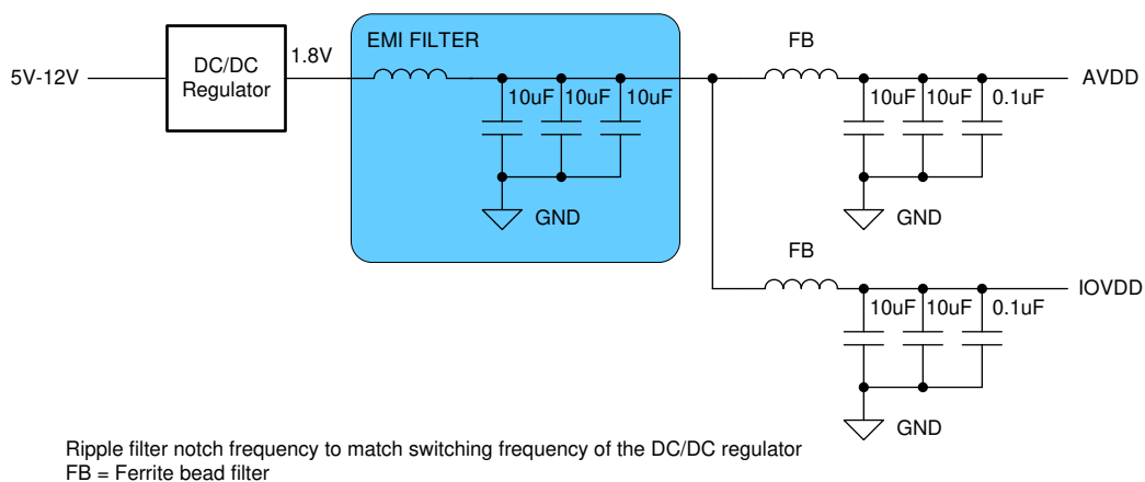
图 11-3. Example Switcher-Only Approach
