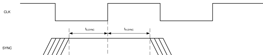
图 8-34. External SYNC timing diagram
