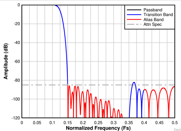
图 8-26. Decimation by 4 complex frequency response
