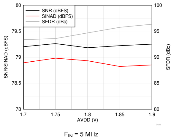
图 6-14. AC Performance vs AVDD
