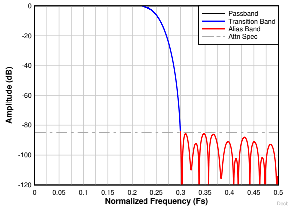
图 8-24. Decimation by 2 complex frequency response
