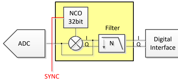
图 8-18. Internal Digital Decimation Filter
