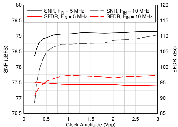
图 6-13. AC Performance vs Clock Amplitude
