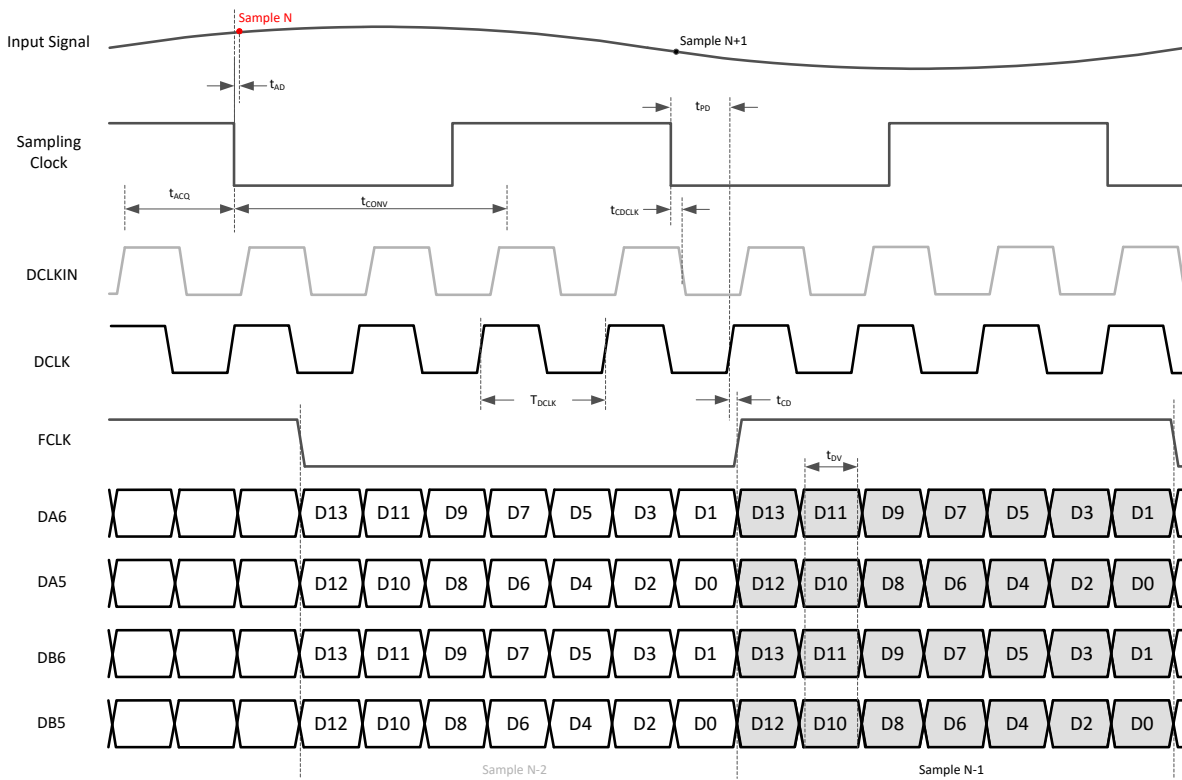
图 7-2. Timing diagram: 2-wire serial CMOS
