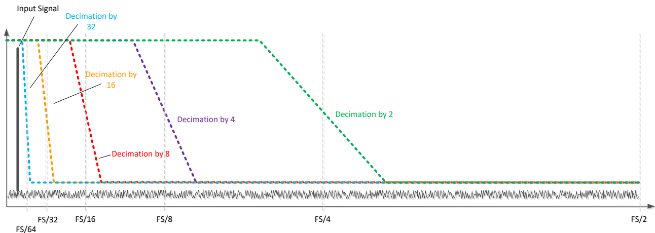
图 8-21. Real decimation illustration
