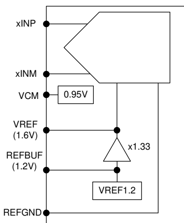
图 8-14. Different voltage reference options for ADC364x
