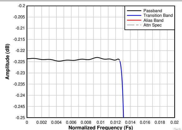
图 8-33. Decimation by 32 complex passband ripple response
