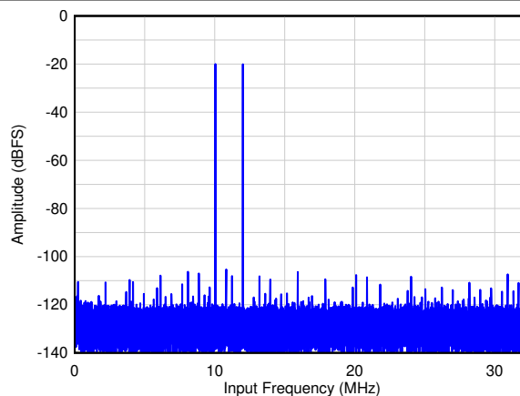
图 6-8. Two Tone FFT at F_{IN} = 10/12 MHz
