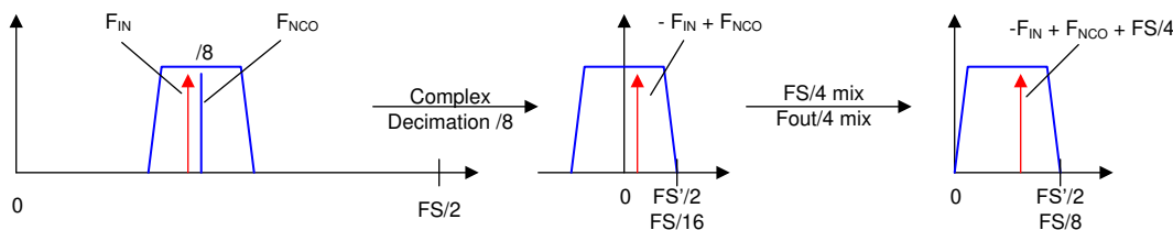
图 8-22. FS/4 Mixing with real output
