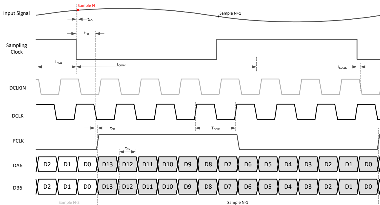
图 7-3. Timing diagram: 1-wire serial CMOS
