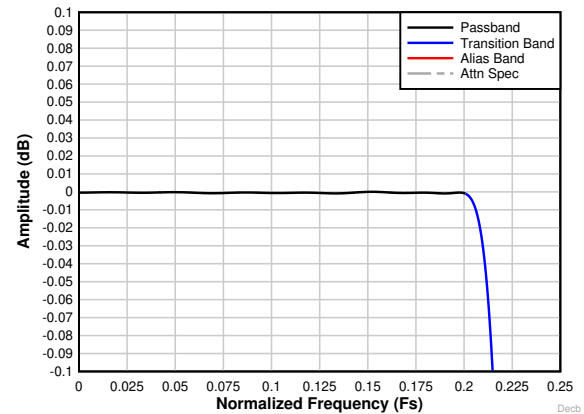
图 8-25. Decimation by 2 complex passband ripple response
