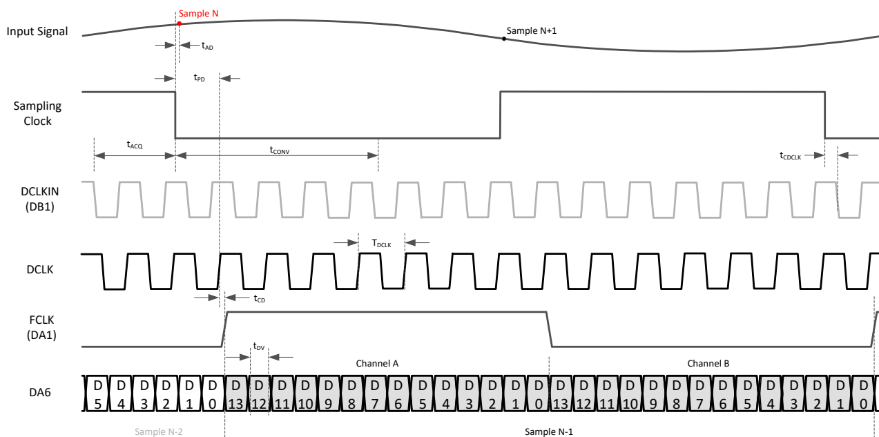
图 7-4. Timing diagram: 1/2-wire serial CMOS
