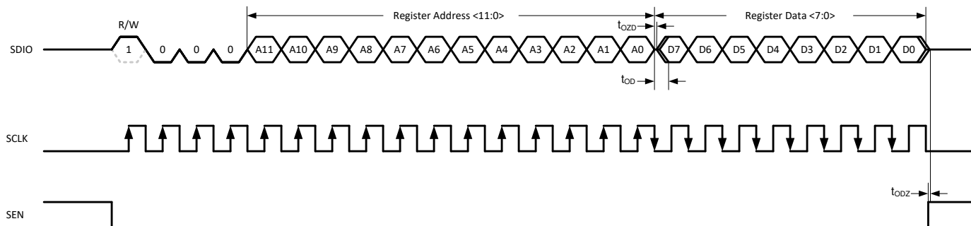
图 8-42. Serial Register Read Timing Diagram
