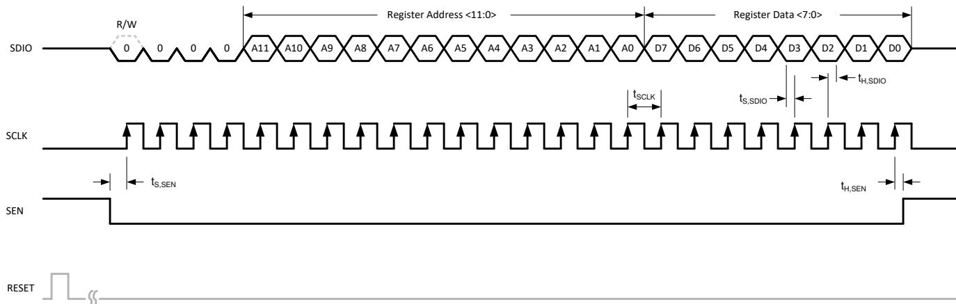
图 8-41. Serial Register Write Timing Diagram
