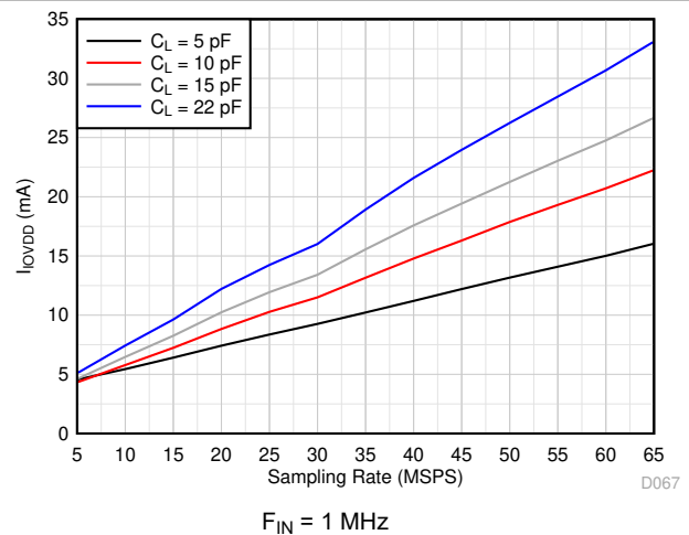
图 6-24. I_{IOVDD} Current vs Load Capacitance
