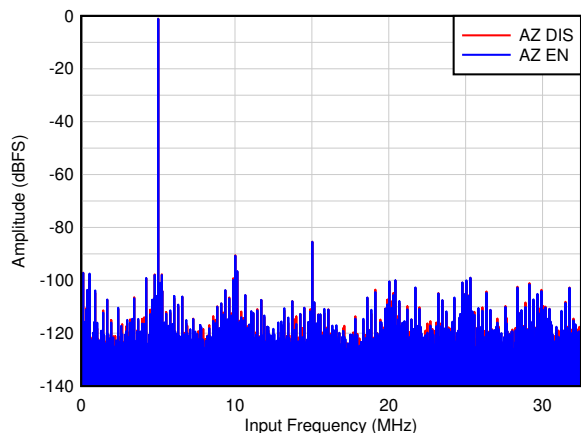
图 8-11. ADC3643: FFT at 65 MSPS with input frequency of 5 MHz (auto-zero feature enable vs disable, 4M point FFT)
