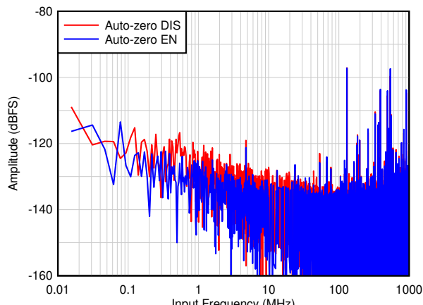
图 8-12. ADC3643: FFT at 65 MSPS with input frequency of 5 MHz (auto-zero feature enabled vs disabled, 4M point FFT)
