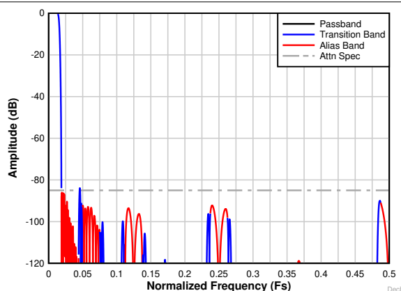
图 8-32. Decimation by 32 complex frequency response
