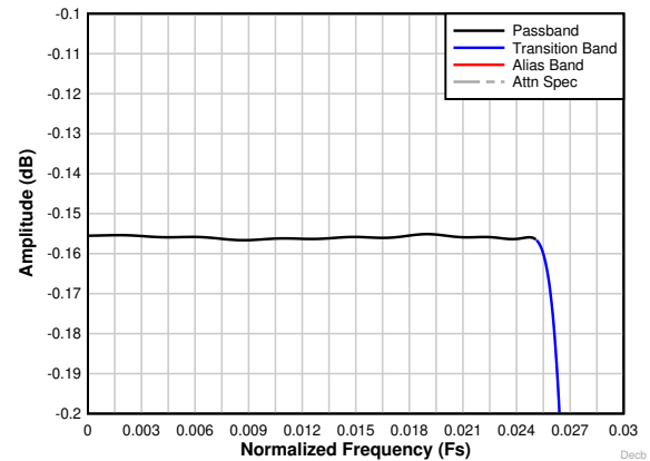
图 8-31. Decimation by 16 complex passband ripple response
