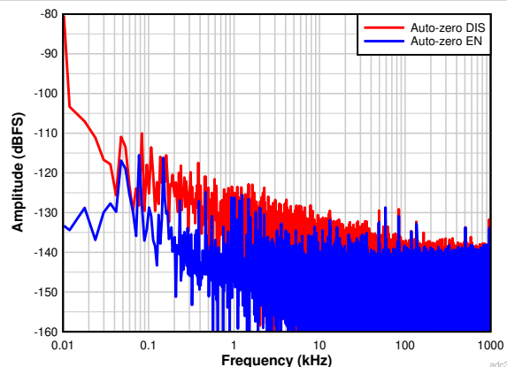
图 8-10. FFT at 25 MSPS with input frequency of 3 MHz (auto-zero feature enable vs disable, 4M point FFT)
