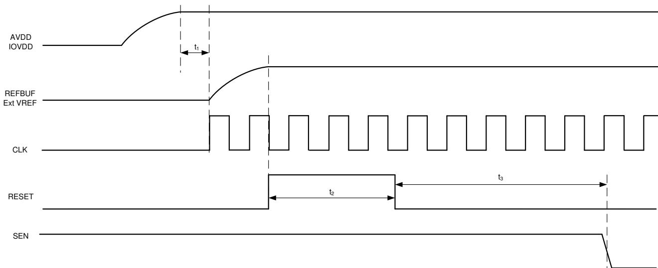
图 10-1. Initialization of serial registers after power up
