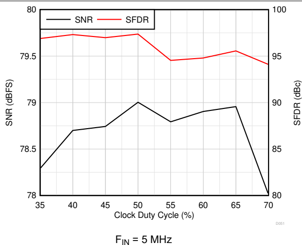
图 6-16. AC Performance vs Clock Duty Cycle
