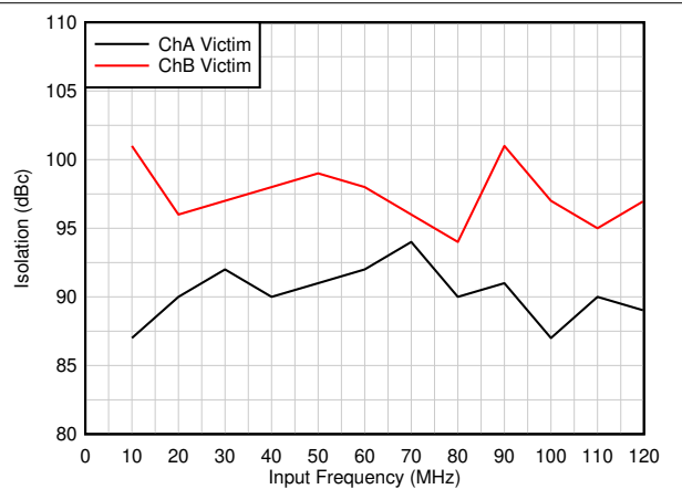
图 6-17. Isolation vs Input Frequency
