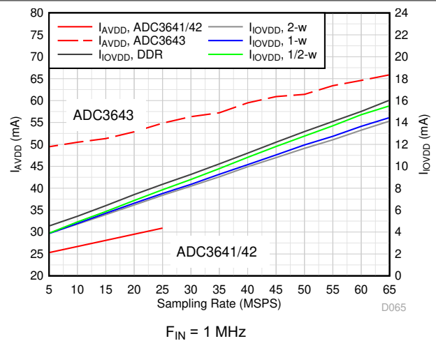
图 6-22. Current vs Sampling Rate
