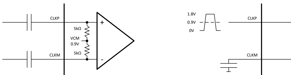
图 8-13. External and internal connection using differential (left) and single ended (right) clock input
