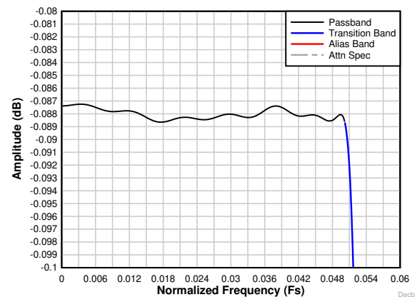
图 8-29. Decimation by 8 complex passband ripple response
