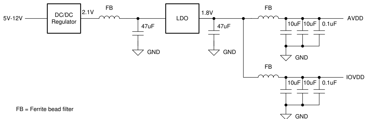
图 11-2. Example: LDO Linear Regulator Approach
