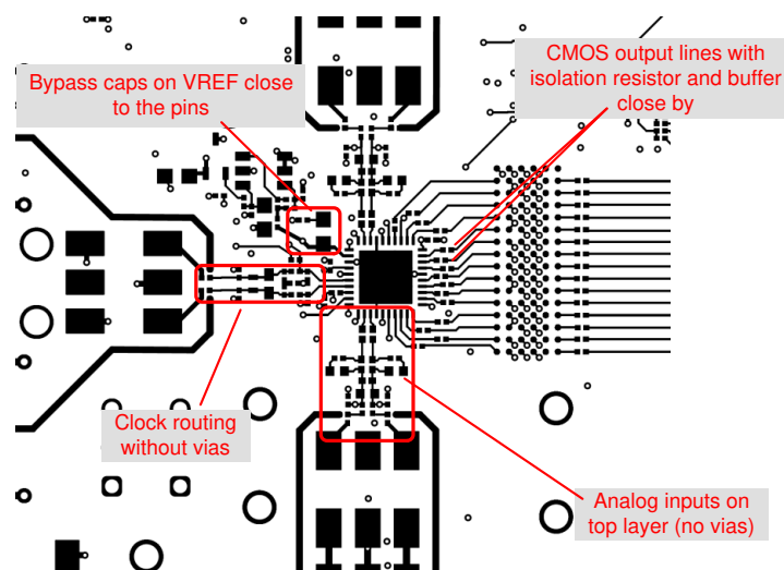
图 12-1. Layout example: top layer of ADC364x EVM
