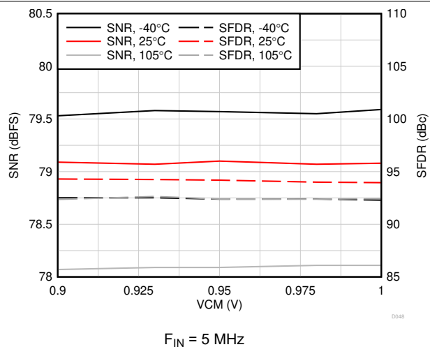
图 6-15. AC Performance vs VCM vs Temperature
