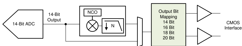
图 8-39. Interface output bit mapper
