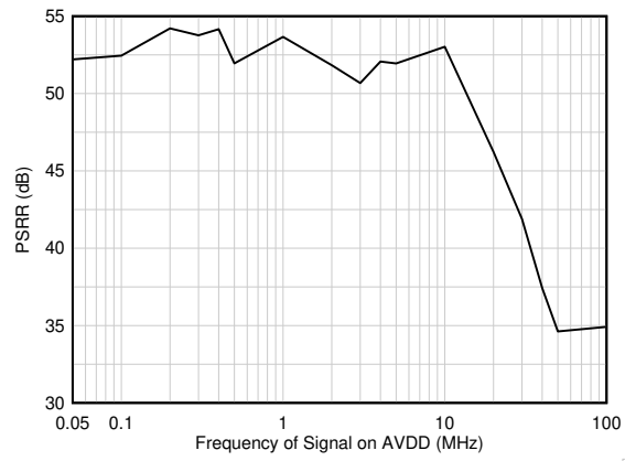
图 11-1. Power supply rejection ratio (PSRR) vs frequency
