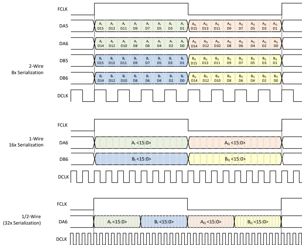
图 8-36. Output Data Format in Complex Decimation
