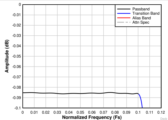
图 8-27. Decimation by 4 complex passband ripple response
