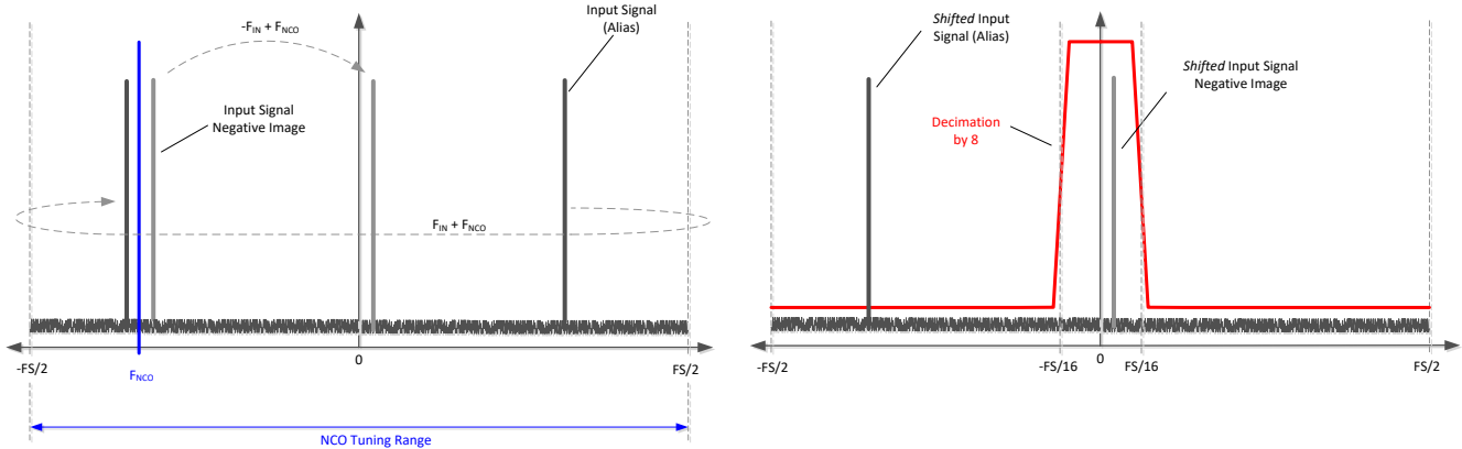
图 8-20. Complex decimation illustration
