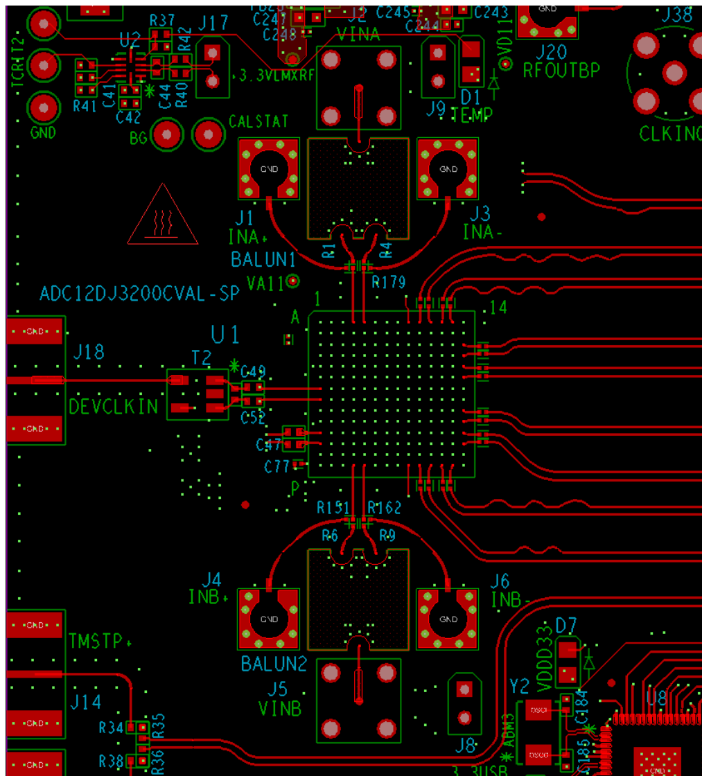
图 197. Top Layer Routing: Analog Inputs, CLK and SYSREF, DA0-3, DB0-3
