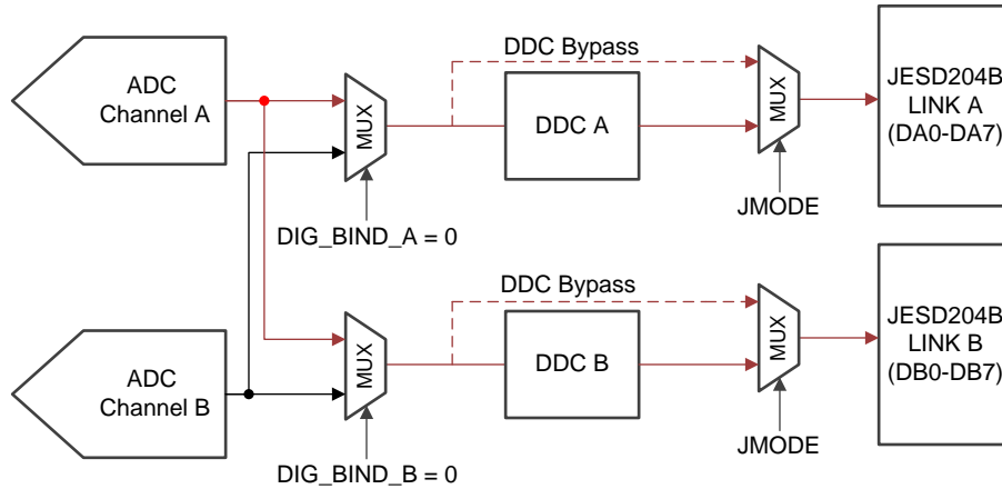
图 93. Dual DDC Mode or Redundant Data Mode for Channel A
