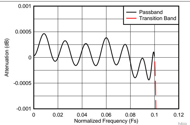
图 82. Decimate-by-2 Composite Zoomed Pass-Band Response (D2_HIGH_PASS = 1)
