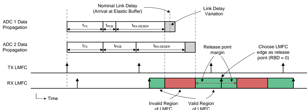
图 92. LMFC Valid Region Definition for Elastic Buffer Release Point Selection
