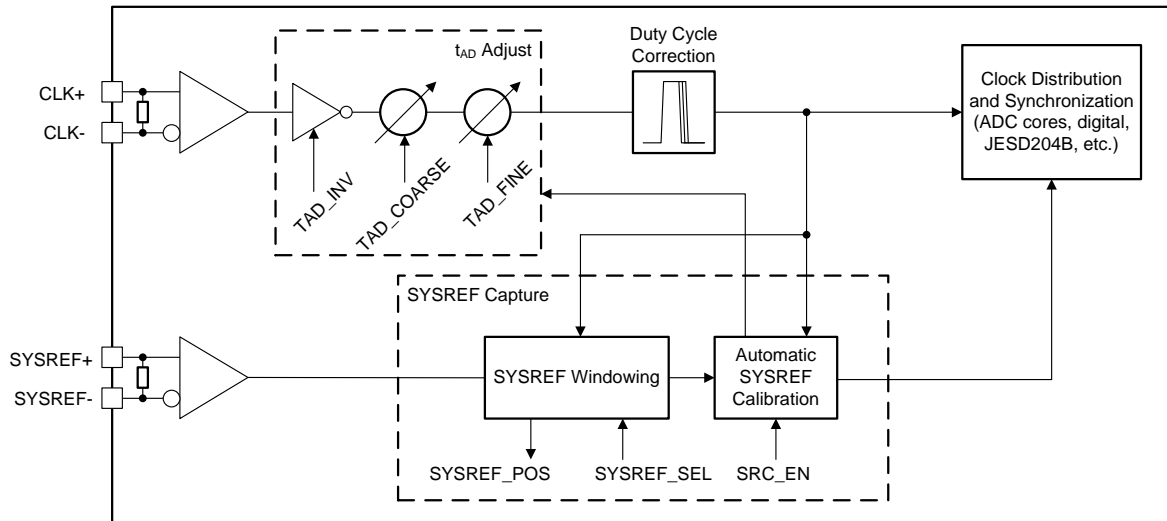
图 75. ADC12DJ3200QML-SP Clocking Subsystem
