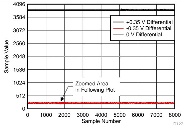
Figure 71. Background Calibration Core Transition (DC Signal)
