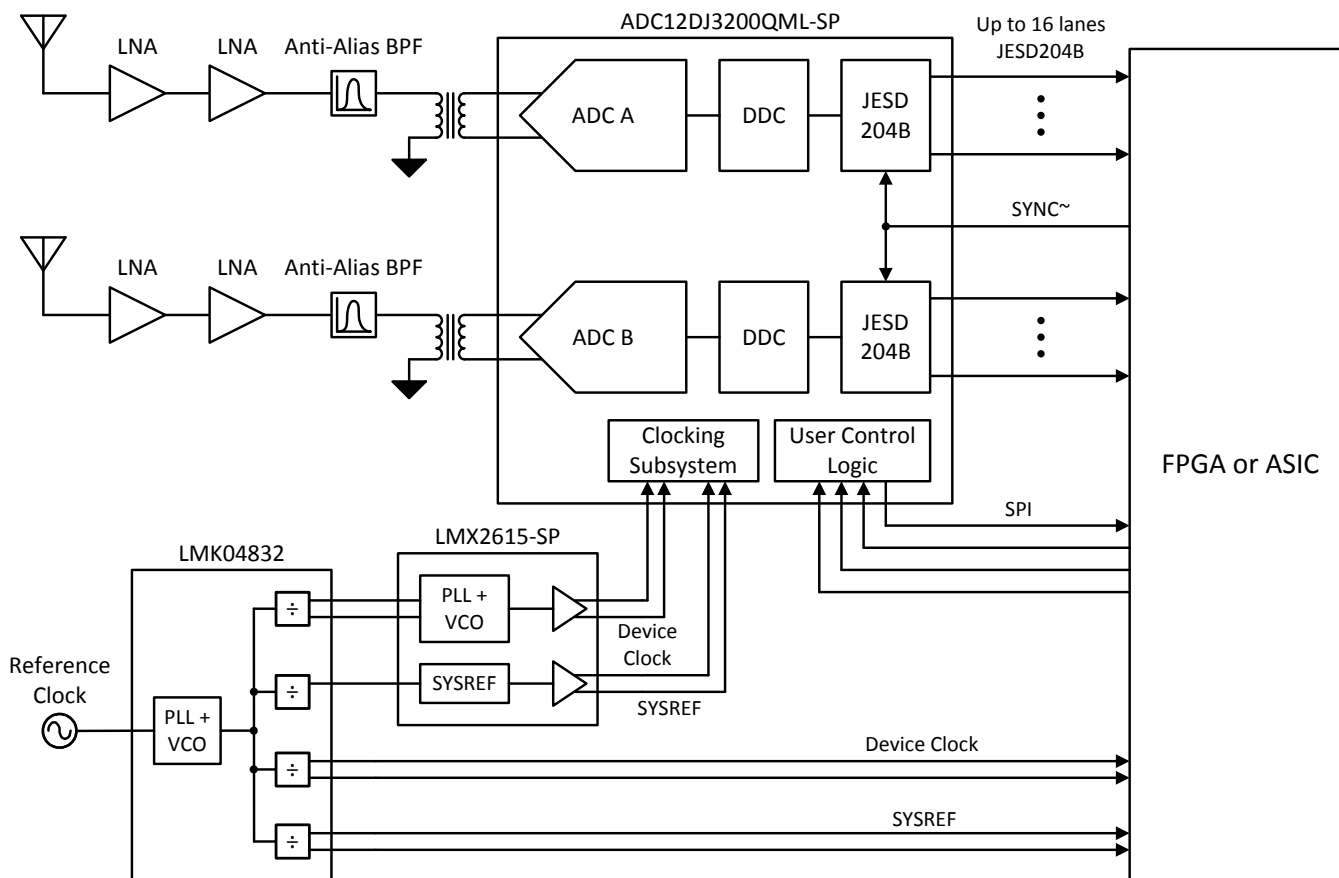
图 190. Typical Configuration for Wideband RF Sampling Receiver
