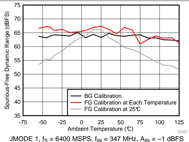
Figure 57. SFDR vs Temperature and Calibration Mode
