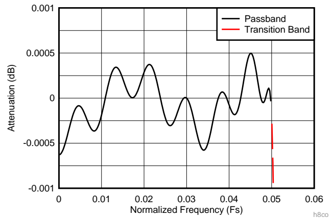
图 86. Decimate-by-4 Composite Zoomed Pass-Band Response (D4_AP87 = 1)
