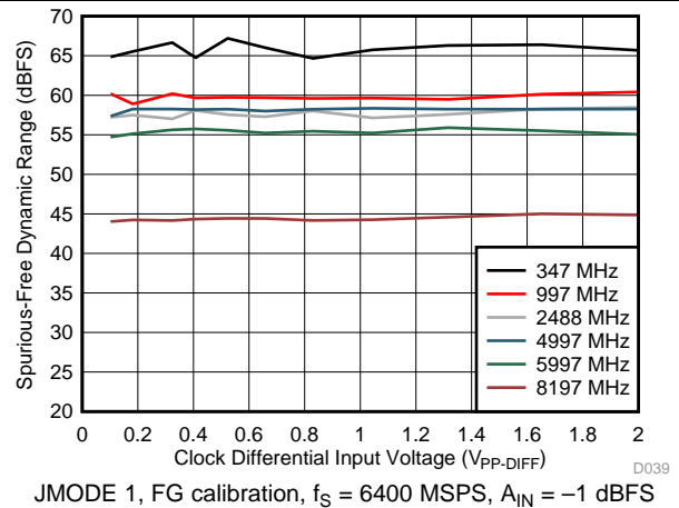
Figure 29. SFDR vs Clock Amplitude
