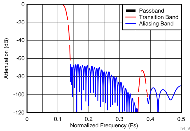
图 85. Decimate-by-4 Composite Response (D4_AP87 = 1)
