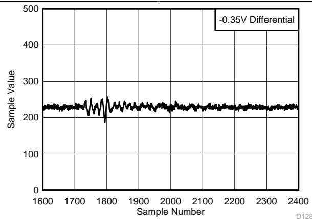
Figure 71. Background Calibration Core Transition (DC Signal)
