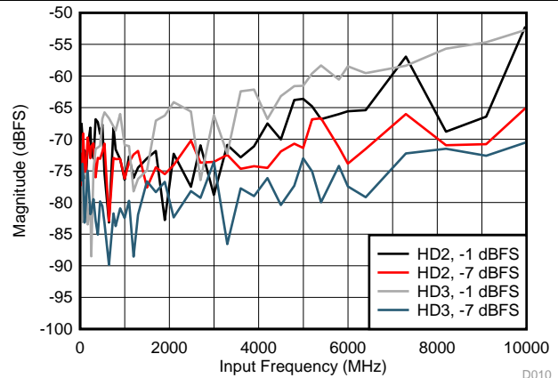
JMODE 1, f_s = 6400\text{ MHz} , FG calibration
