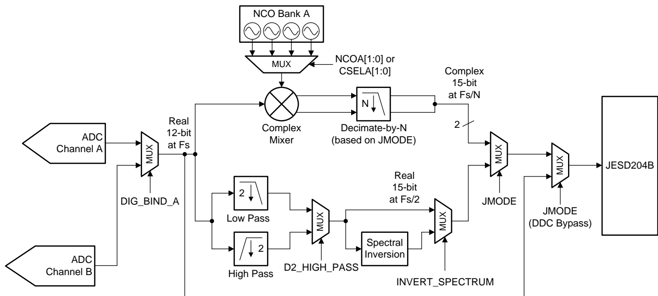
图 77. Channel A Digital Down Conversion Block (Dual-Channel Mode Only)
