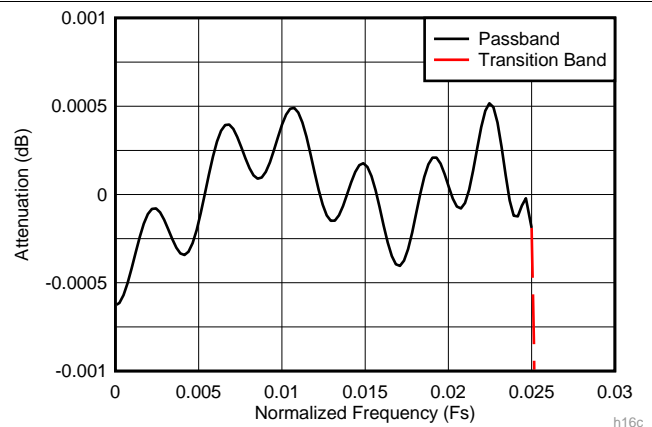
图 88. Decimate-by-8 Composite Zoomed Pass-Band Response
