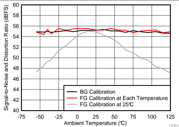
Figure 52. SINAD vs Temperature and Calibration Mode
