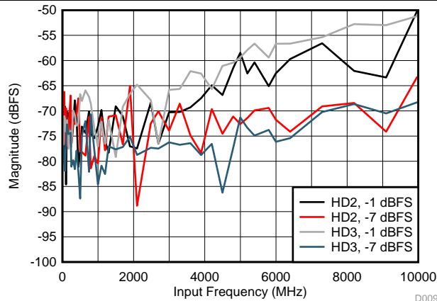
JMODE 3, f_s = 3200\text{ MHz} , FG calibration
