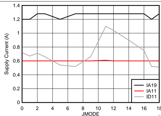
Figure 65. Supply Current vs JMODE
