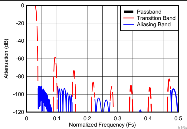
图 89. Decimate-by-16 Composite Response
