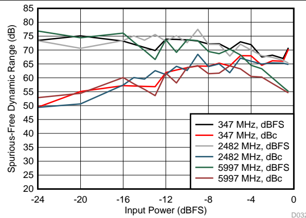
JMODE 3, FG calibration, f_s = 3200\text{ MSPS}
