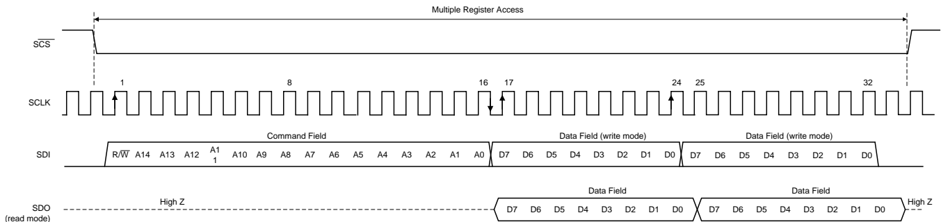
图 97. Serial Interface Protocol: Streaming Read and Write
