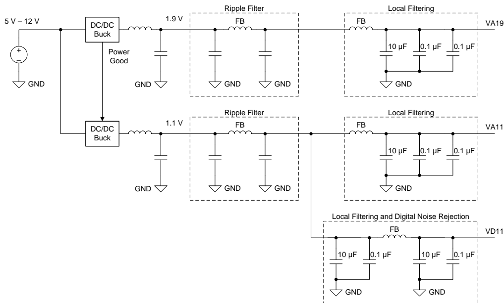
图 196. DC/DC Switching Regulator Example
