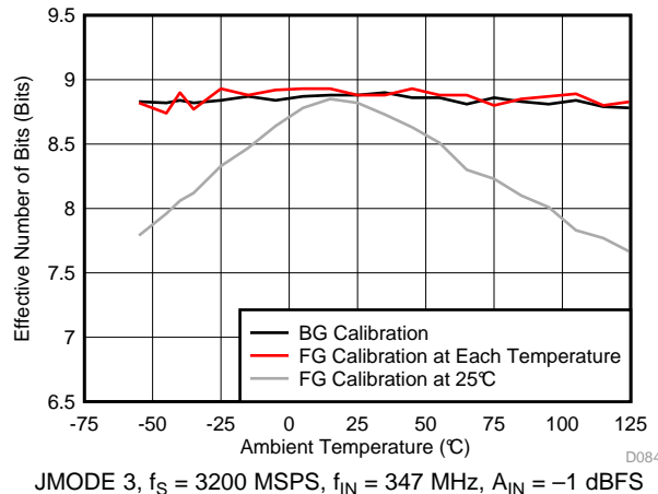
Figure 54. ENOB vs Temperature and Calibration Mode
