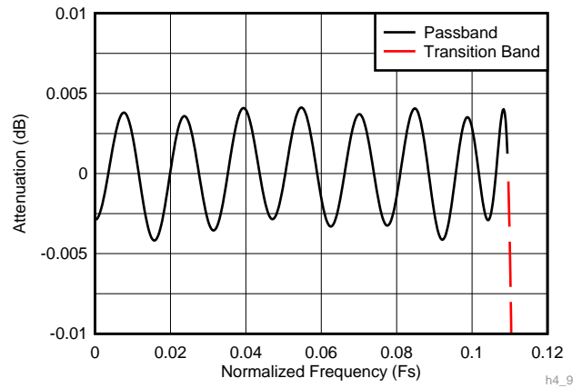
图 86. Decimate-by-4 Composite Zoomed Pass-Band Response (D4_AP87 = 1)
