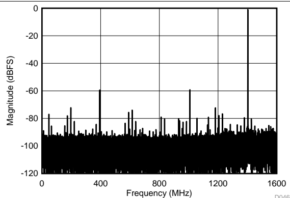
JMODE 3, FG calibration, f_s = 3200\text{ MSPS} , SNR = 53.0 dBFS, SFDR = 59 dBFS, ENOB = 8.2 bits
