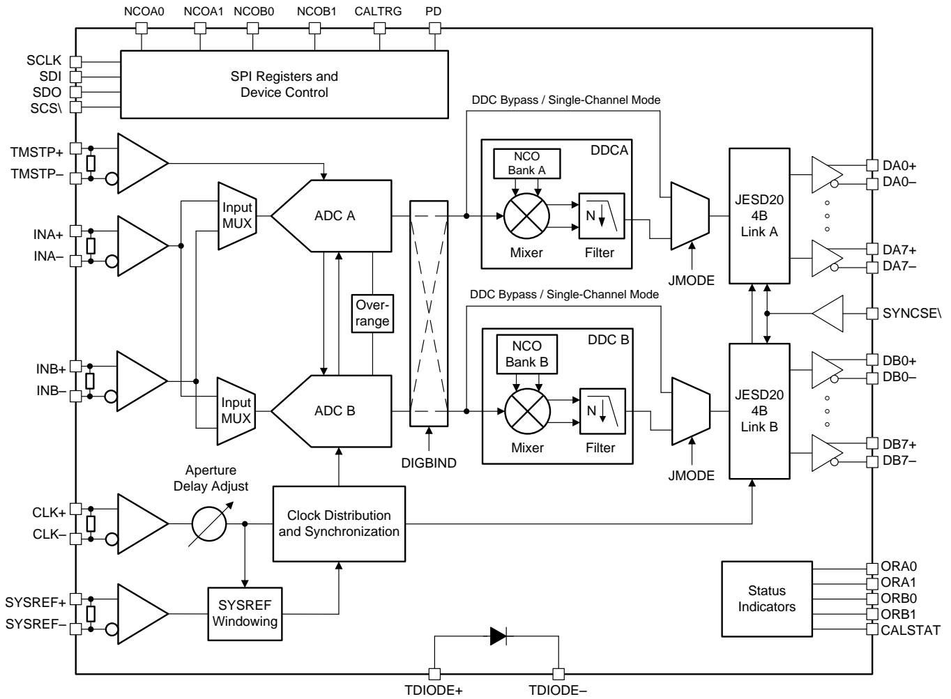
图 73. Functional Block Diagram
