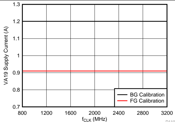
JMODE 1, f_{\text{IN}} = 2482\text{ MHz} , A_{\text{IN}} = -1\text{ dBFS}
