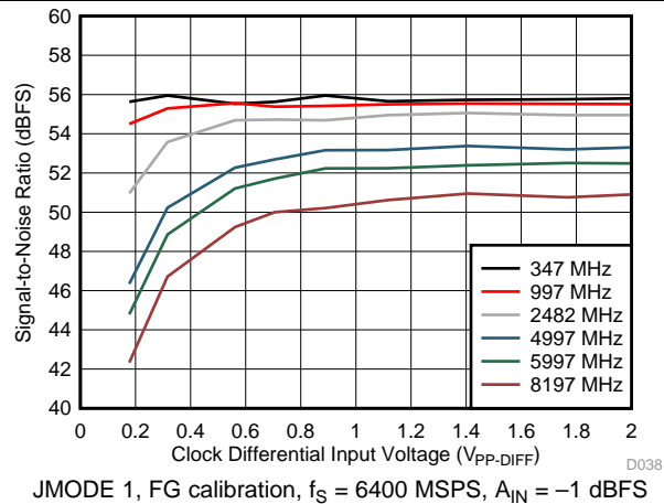
Figure 28. SNR vs Clock Amplitude
