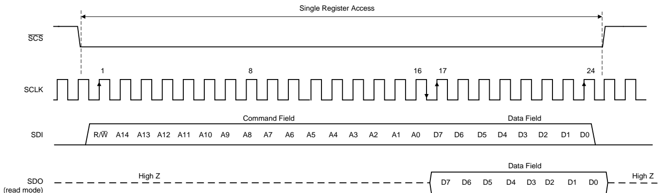
图 96. Serial Interface Protocol: Single Read/Write
