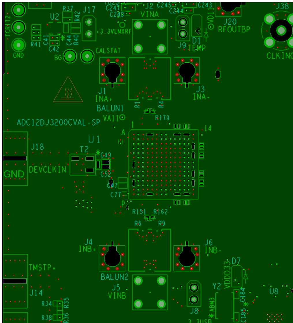
图 198. GND1 Cutouts to Optimize Impedance of Component Pads
