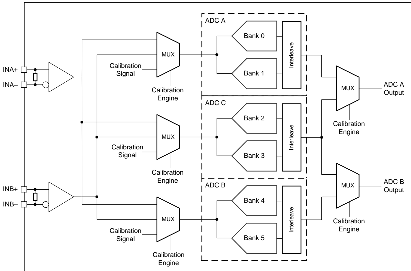
图 95. ADC12DJ3200QML-SP Calibration System Block Diagram
