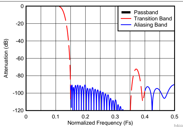
图 81. Decimate-by-2 Composite Response (D2_HIGH_PASS = 1)
