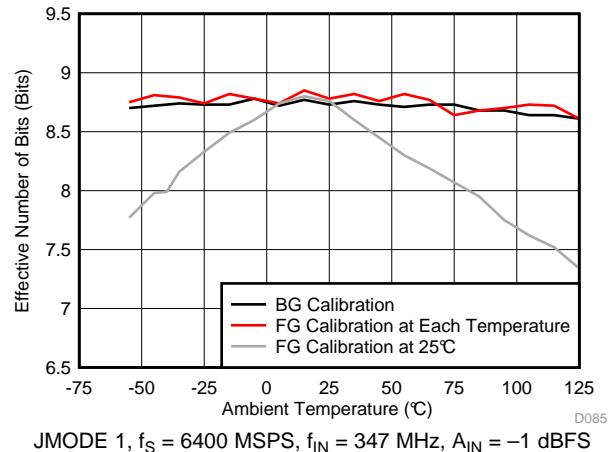
Figure 55. ENOB vs Temperature and Calibration Mode
