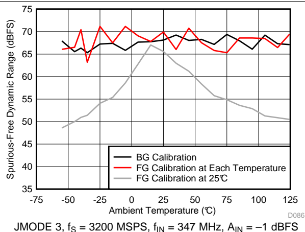
Figure 56. SFDR vs Temperature and Calibration Mode
