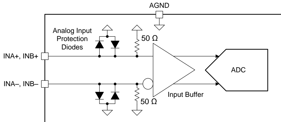
图 74. ADC12DJ3200QML-SP Analog Input Internal Termination and Protection Diagram
