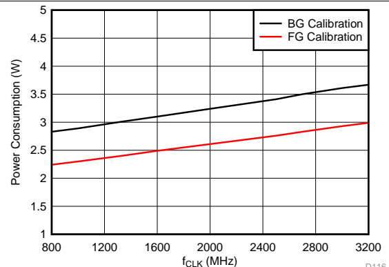
JMODE 1, f_{\text{IN}} = 2482\text{ MHz} , A_{\text{IN}} = -1\text{ dBFS}
