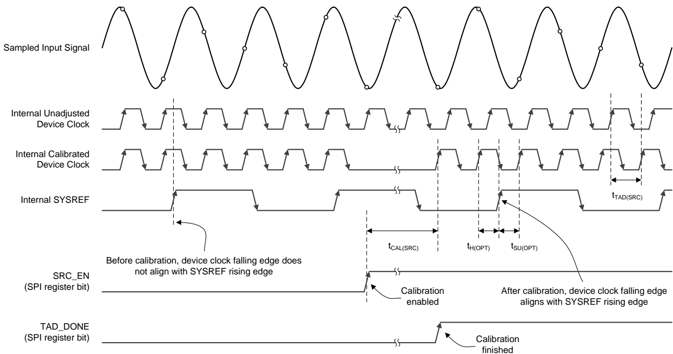
图 76. SYSREF Calibration Timing Diagram
