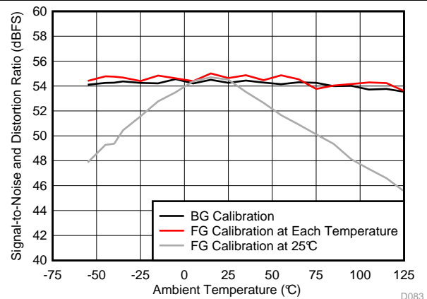
Figure 53. SINAD vs Temperature and Calibration Mode
