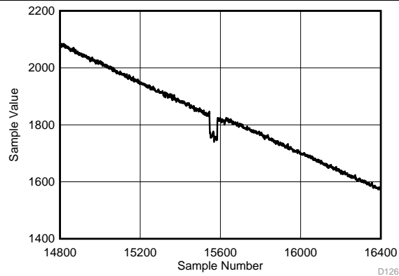
Figure 70. Background Calibration Core Transition (AC Signal Zoomed)
