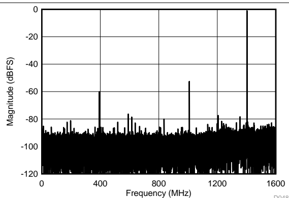
JMODE 3, FG calibration, f_s = 3200\text{ MSPS} , SNR = 51.1 dBFS, SFDR = 53 dBFS, ENOB = 7.8 bits
