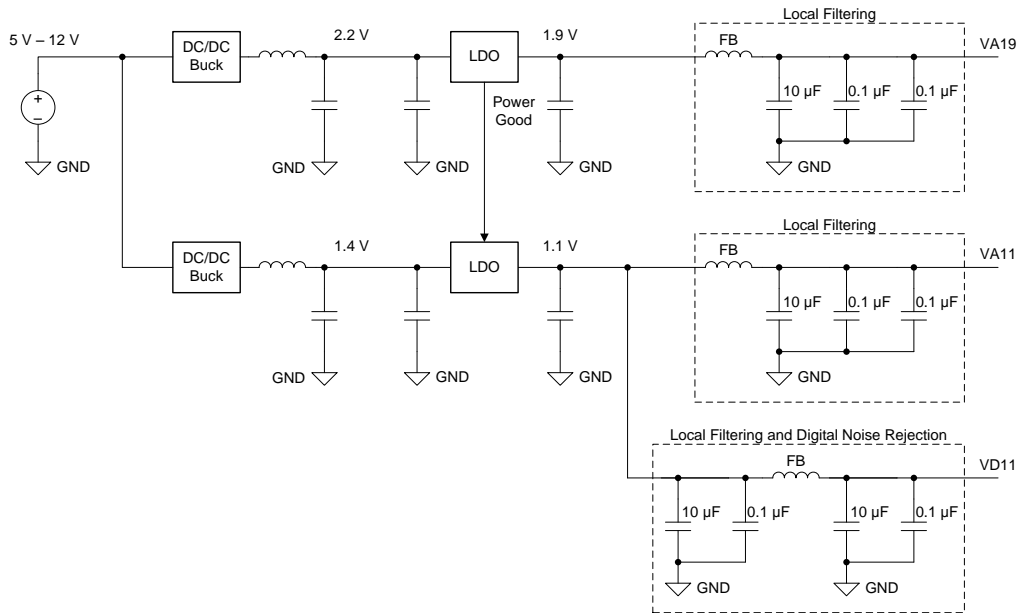
图 195. LDO Linear Regulator Example
