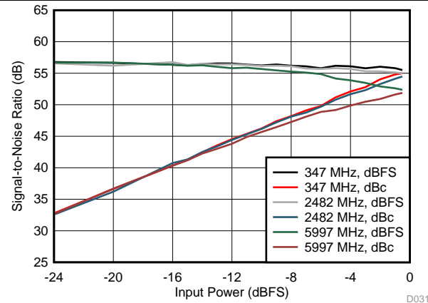
JMODE 1, FG calibration, f_s = 6400\text{ MSPS}
