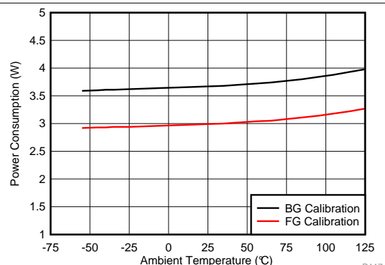
Figure 67. Power Consumption vs Temperature
