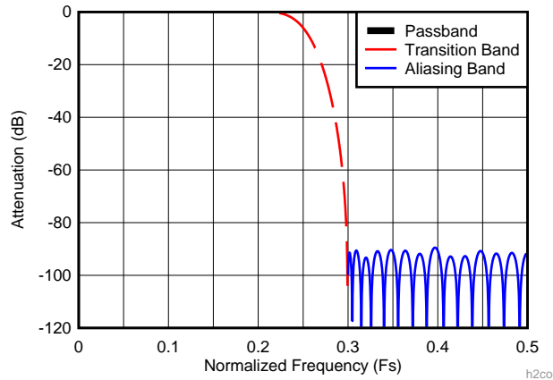
图 79. Decimate-by-2 Composite Response (D2_HIGH_PASS = 0)
