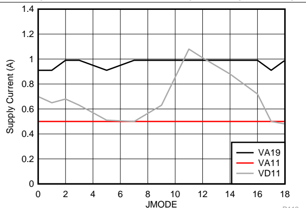
Figure 64. Supply Current vs JMODE
