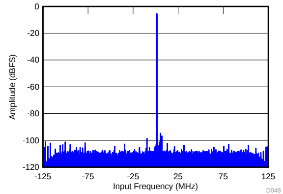
Figure 49. FFT for 370-MHz Input Signal
