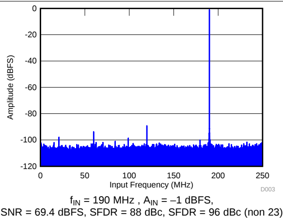
Figure 4. FFT for 190-MHz Input Signal
