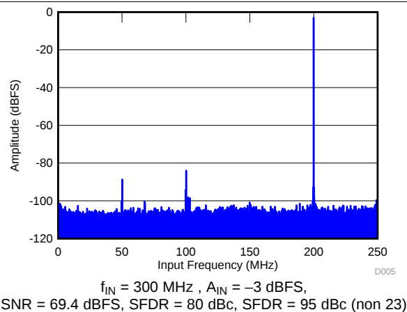
Figure 6. FFT for 300-MHz Input Signal
