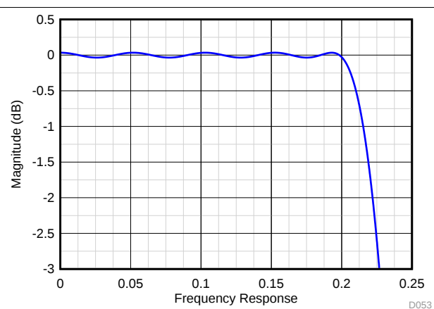
Figure 55. Zoomed View of Frequency Response
