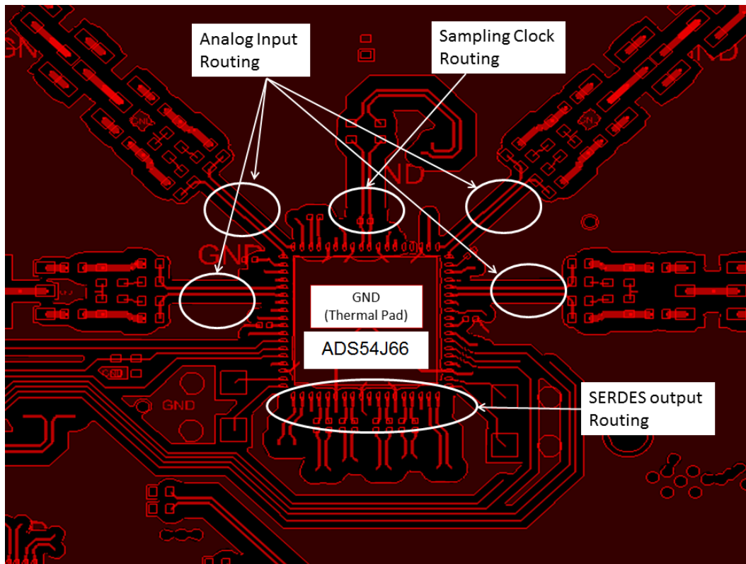
Figure 147. ADS54J66EVM Layout
