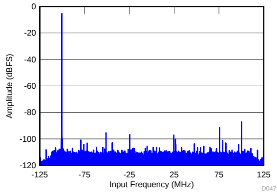
Figure 48. FFT for 270-MHz Input Signal
