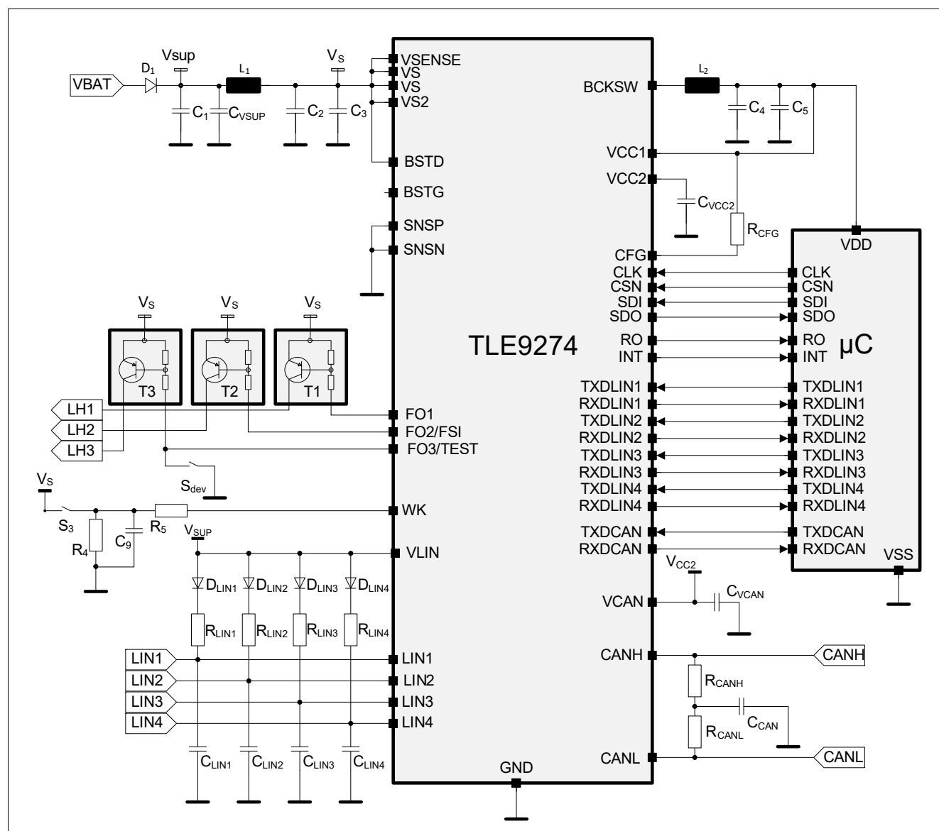
Figure 51 Application Diagram
