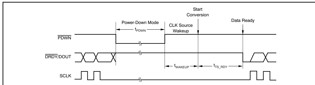
Figure 9. Wake-Up Timing from Power-Down Mode
