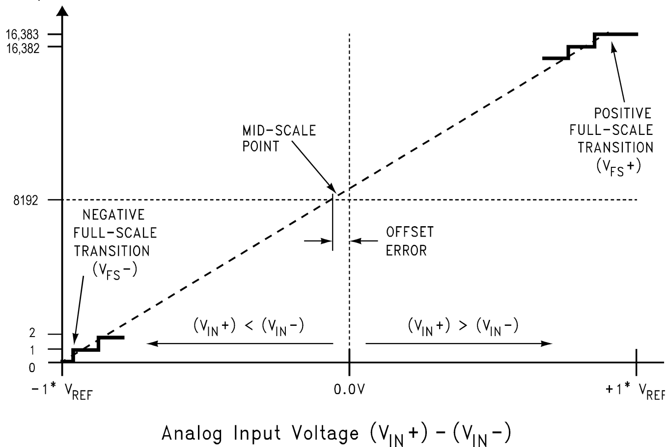
Figure 2. Transfer Characteristic
