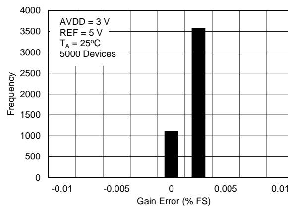
Figure 41. TYPICAL DISTRIBUTION OF GAIN ERROR
