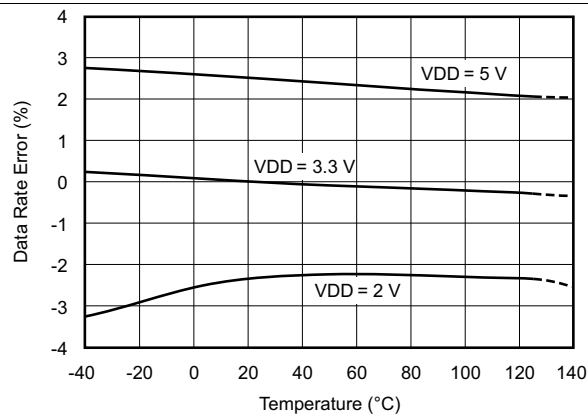
Figure 20. Data Rate vs Temperature
