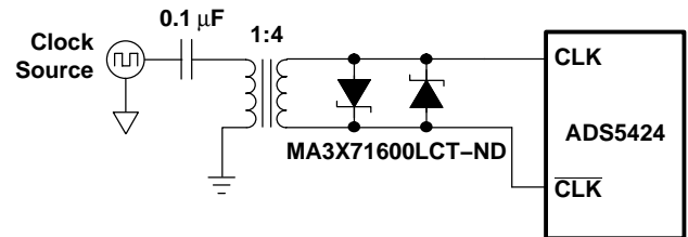
Figure 44. Differential Clock
