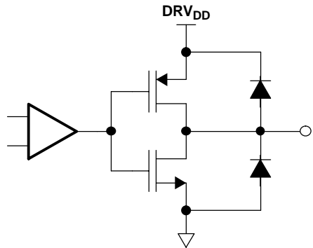
Figure 33. Digital Output
