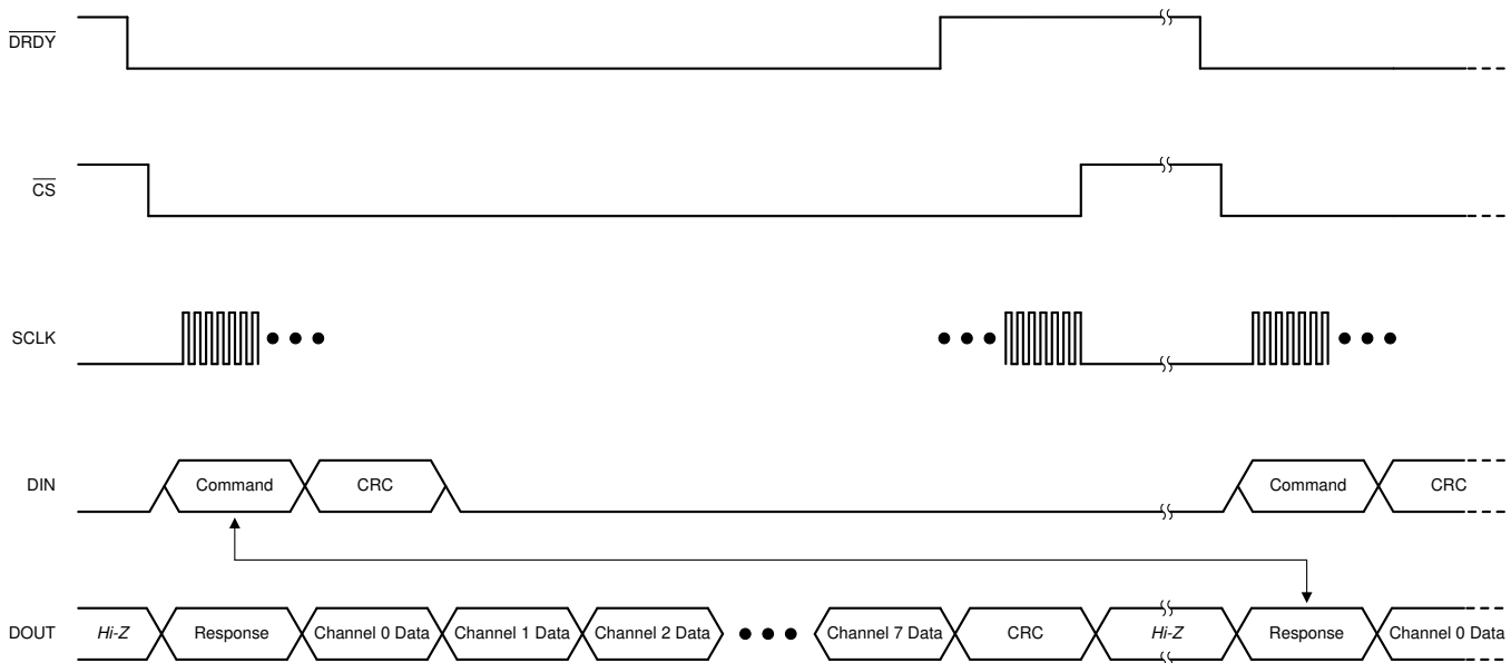
图 40. Typical Communication Frame
