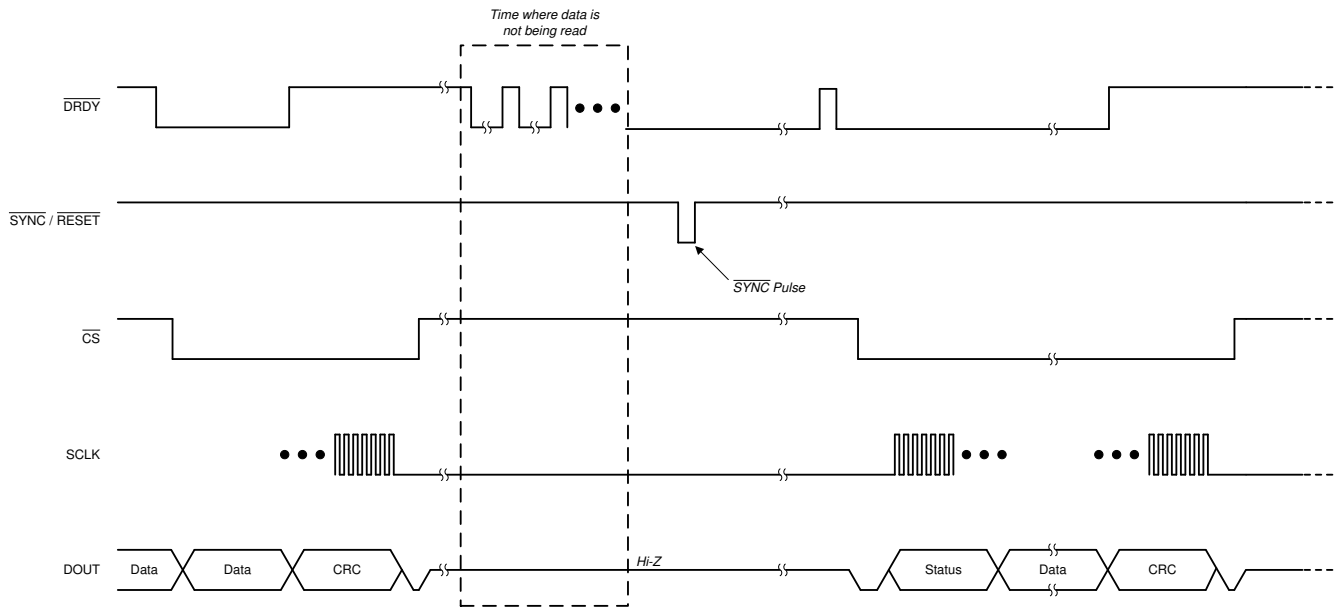
图 42. Collecting Data After a Hiatus Using the SYNC/RESET Pin
