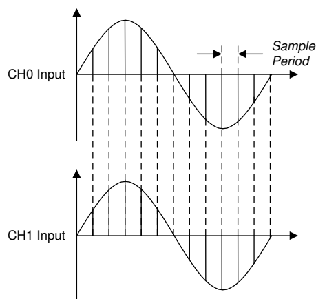
图 33. Two Channel Outputs With Equal Phase Settings
