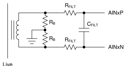
图 105. Current Measurement Front-End
