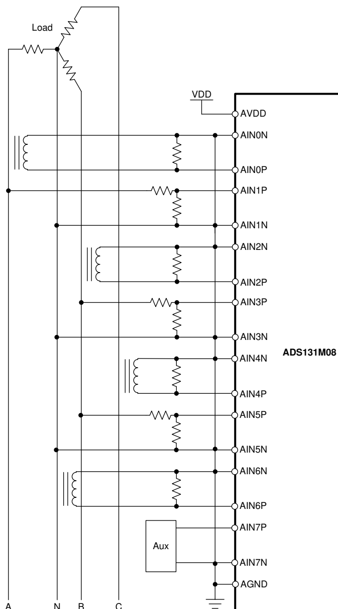
图 103. Three-Phase Metrology Design Front-End
