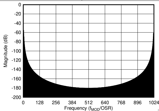
图 28. Sinc³ Digital Filter Response, OSR 1024, Stop-Band Detail
