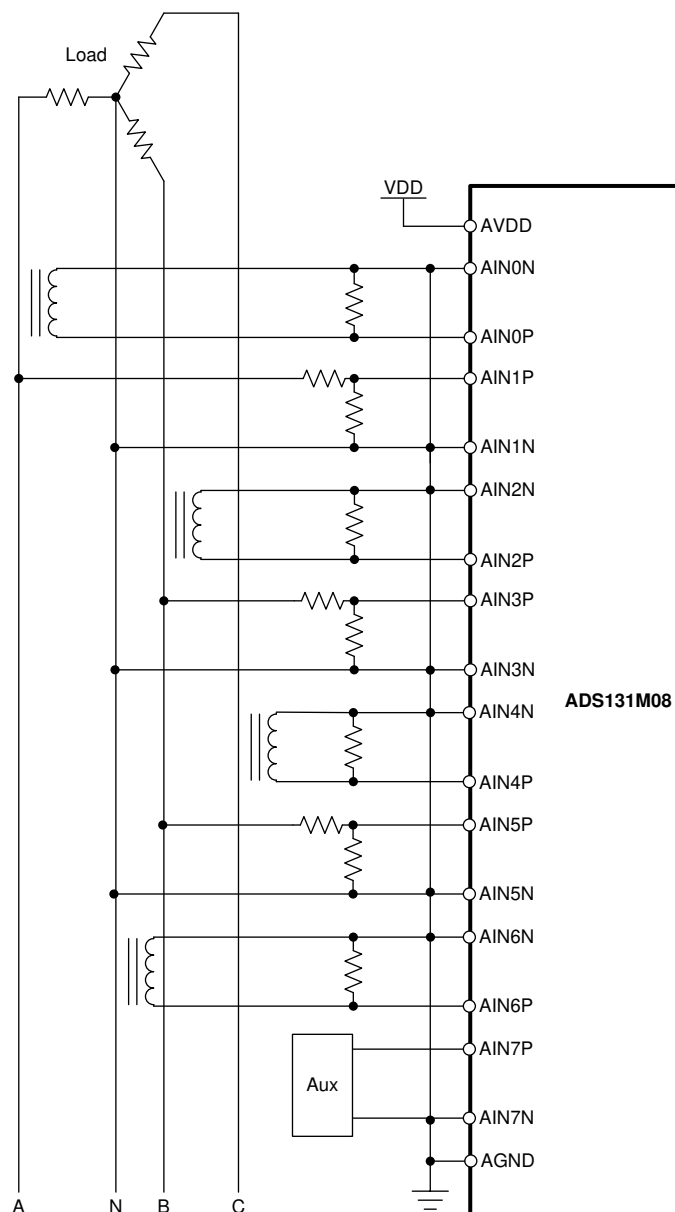
图 101. Three-Phase Current and Voltage Measurement Front-End With a Neutral Current Monitor
