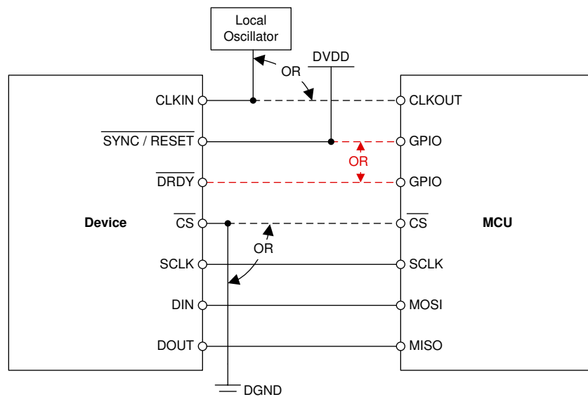
图 100. Minimum Connections Required to Operate the ADS131M08
