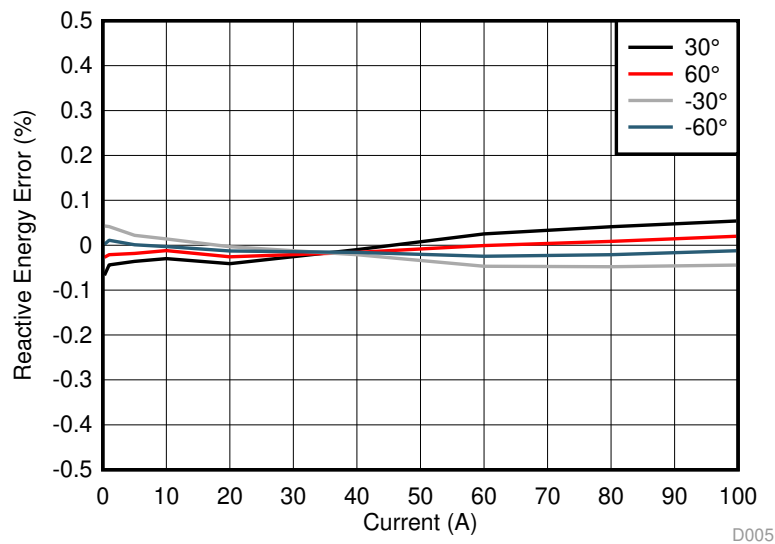
图 107. Cumulative Reactive Energy % Error Versus Current
