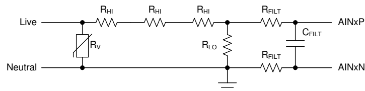
图 104. Voltage Measurement Front-End
