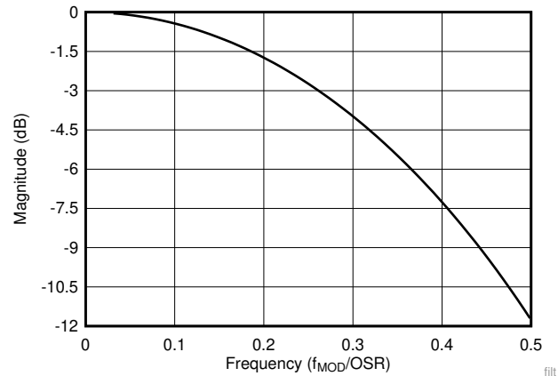
图 27. Sinc³ Digital Filter Response, Pass-Band Detail
