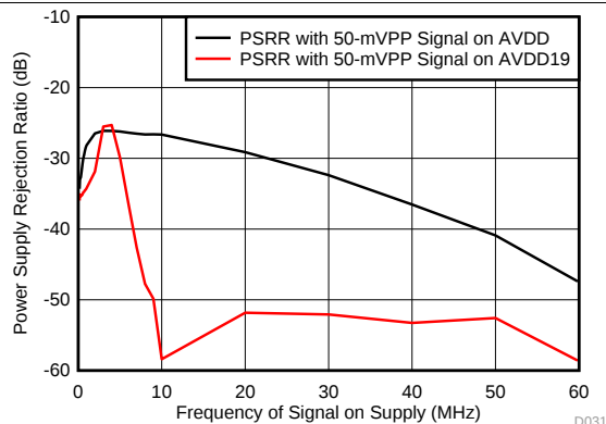
图 32. PSRR vs Power-Supply Noise Frequency
