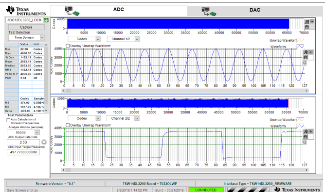
图 177. 200-MHz, Sine-Wave (Channel A) and 40-MHz, Square-Wave (Channel B) Time Domain for 5-GSPS, Single-Channel Oscilloscope
