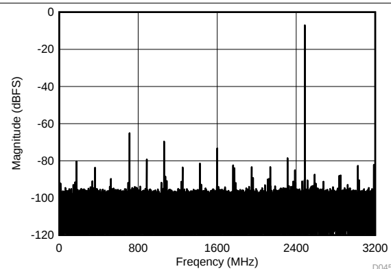
Figure 41. Single-Tone FFT at f_{\text{IN}} = 2488 \text{ MHz} , A_{\text{IN}} = -7 \text{ dBFS}
