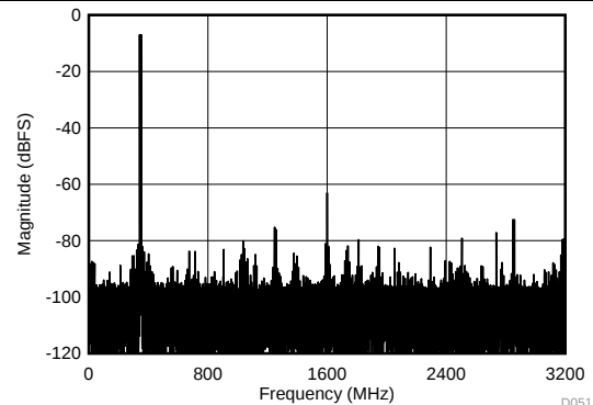
DES_EN = 1, FG calibration, f_s = 6400\text{ MSPS} , f_1 = 342\text{ MHz} , f_2 = 352\text{ MHz} , A_{\text{IN}} = -7\text{ dBFS} per tone, SFDR = -73\text{ dBFS} , IMD3 = -81\text{ dBFS} , IMD2 = -88\text{ dBFS}
