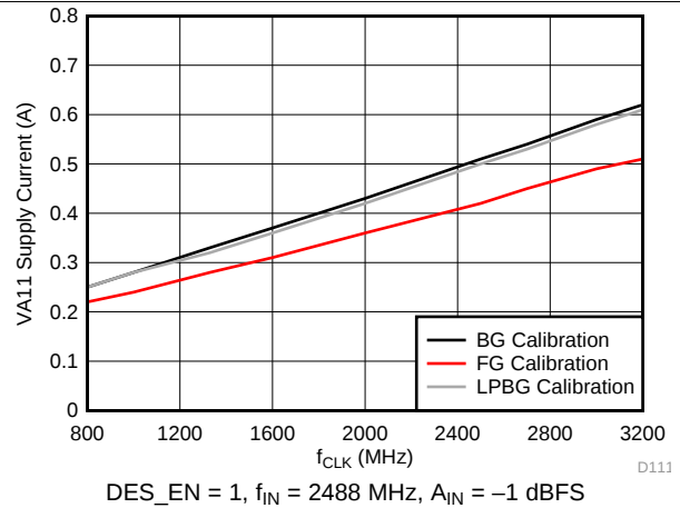
Figure 67. VA11 Supply Current vs Clock Rate
