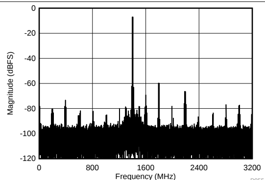
DES_EN = 1, FG calibration, f_s = 6400\text{ MSPS} , f_1 = 4992\text{ MHz} , f_2 = 5002\text{ MHz} , A_{\text{IN}} = -7\text{ dBFS} per tone, SFDR = -60\text{ dBFS} , IMD3 = -62\text{ dBFS} , IMD2 = -78\text{ dBFS}
