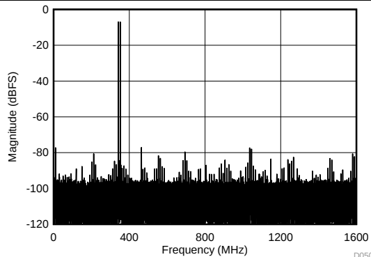
DES_EN = 0, FG calibration, f_s = 3200\text{ MSPS} , f_1 = 342\text{ MHz} , f_2 = 352\text{ MHz} , A_{\text{IN}} = -7\text{ dBFS} per tone, SFDR = -77\text{ dBFS} , IMD3 = -87\text{ dBFS} , IMD2 = -77\text{ dBFS}
