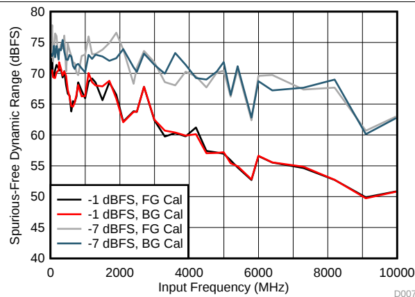
Figure 16. SFDR vs Input Frequency
