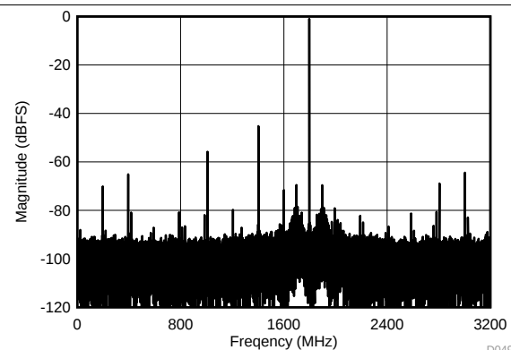
Figure 43. Single-Tone FFT at f_{\text{IN}} = 4997 \text{ MHz} , A_{\text{IN}} = -1 \text{ dBFS}
