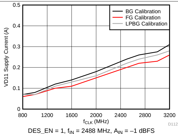
Figure 68. VD11 Supply Current vs Clock Rate
