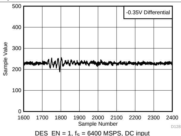
Figure 77. Background Calibration Core Transition (DC Signal Zoomed)
