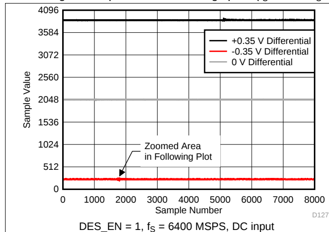
Figure 76. Background Calibration Core Transition (DC Signal)
