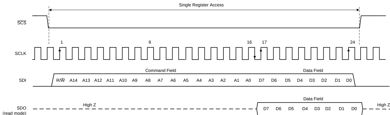
图 82. Serial Interface Protocol: Single Read/Write Operation
