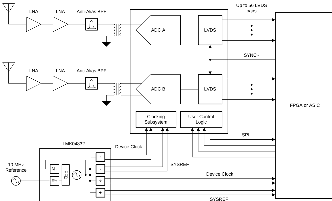
图 168. Typical Configuration for Wideband RF Sampling
