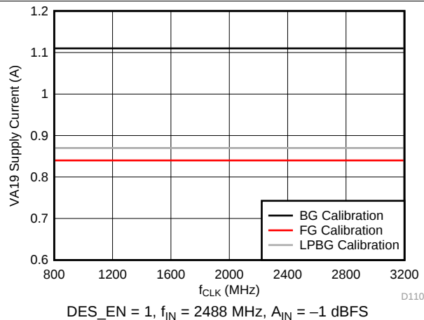
Figure 66. VA19 Supply Current vs Clock Rate
