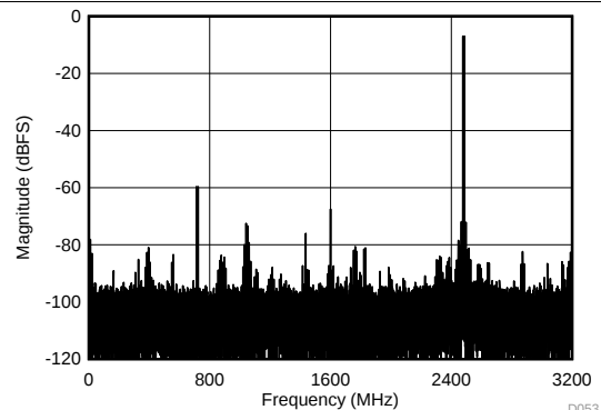
DES_EN = 1, FG calibration, f_s = 6400\text{ MSPS} , f_1 = 2483\text{ MHz} , f_2 = 2493\text{ MHz} , A_{\text{IN}} = -7\text{ dBFS} per tone, SFDR = -60\text{ dBFS} , IMD3 = -72\text{ dBFS} , IMD2 = -78\text{ dBFS}
