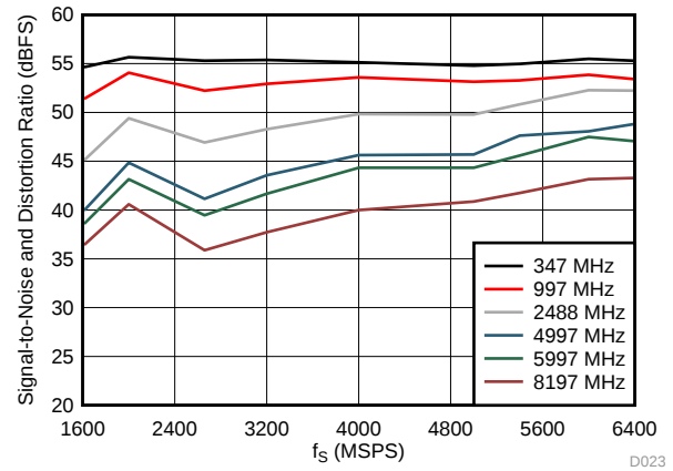
Figure 23. SNR vs Sampling Rate
