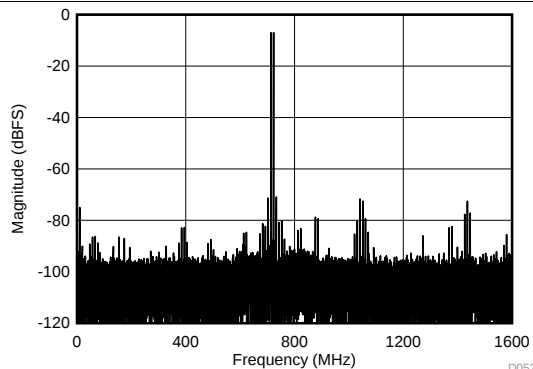
DES_EN = 0, FG calibration, f_s = 3200\text{ MSPS} , f_1 = 2483\text{ MHz} , f_2 = 2493\text{ MHz} , A_{\text{IN}} = -7\text{ dBFS} per tone, SFDR = -71\text{ dBFS} , IMD3 = -71\text{ dBFS} , IMD2 = -75\text{ dBFS}
