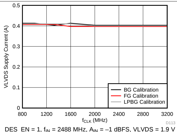
Figure 69. VLVDS Supply Current vs Clock Rate
