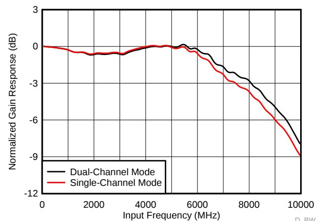
ADC12DL3200 频率响应
