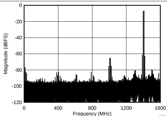
DES_EN = 0, FG calibration, f_s = 3200\text{ MSPS} , f_1 = 4992\text{ MHz} , f_2 = 5002\text{ MHz} , A_{\text{IN}} = -7\text{ dBFS} per tone, SFDR = -61\text{ dBFS} , IMD3 = -61\text{ dBFS} , IMD2 = -77\text{ dBFS}
