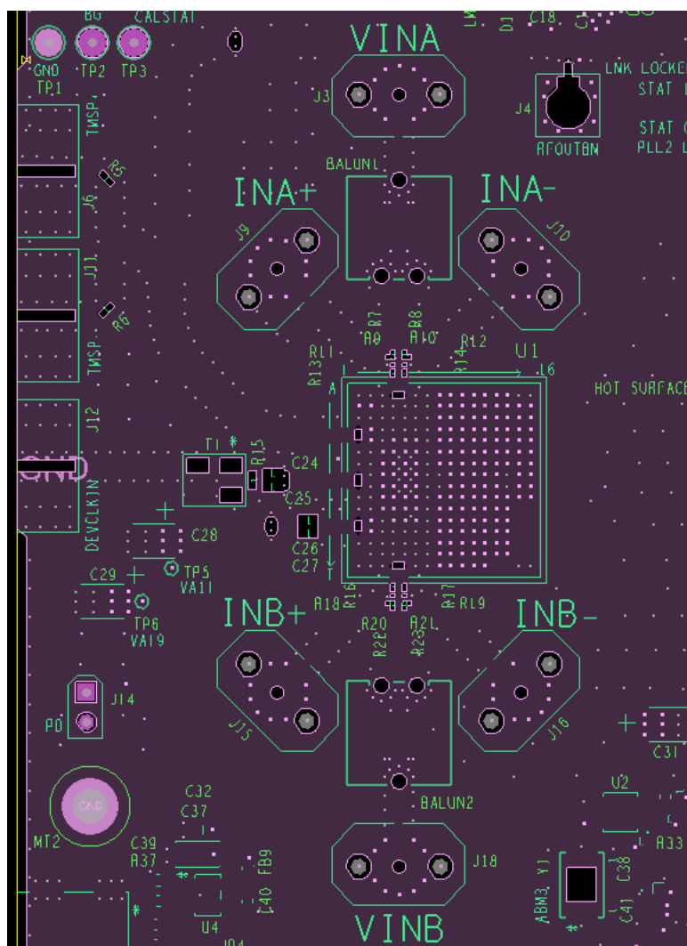
图 182. GND1 Cutouts to Optimize Impedance of Component Pads
