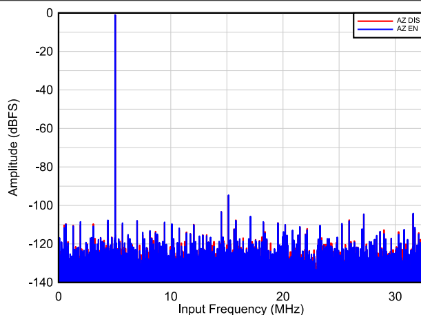
图 8-10. FFT at 65 MSPS with input frequency of 3 MHz (auto-zero feature enable vs disable, 4M point FFT)
