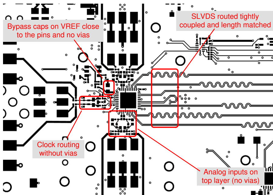
图 11-1. Layout example: top layer of ADC366x/368x EVM
