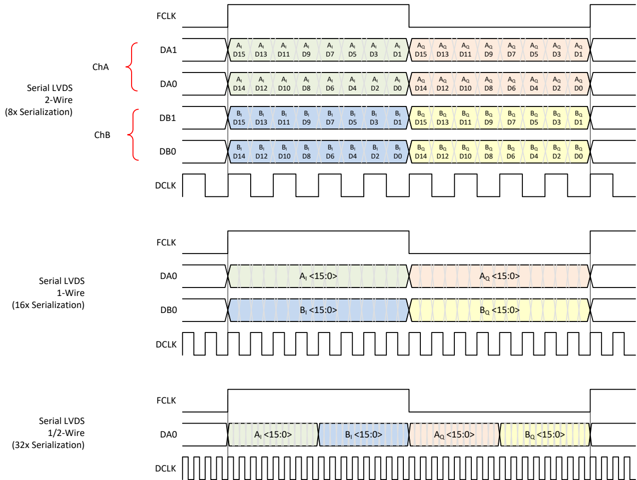
图 8-36. Output Data Format in Complex Decimation
