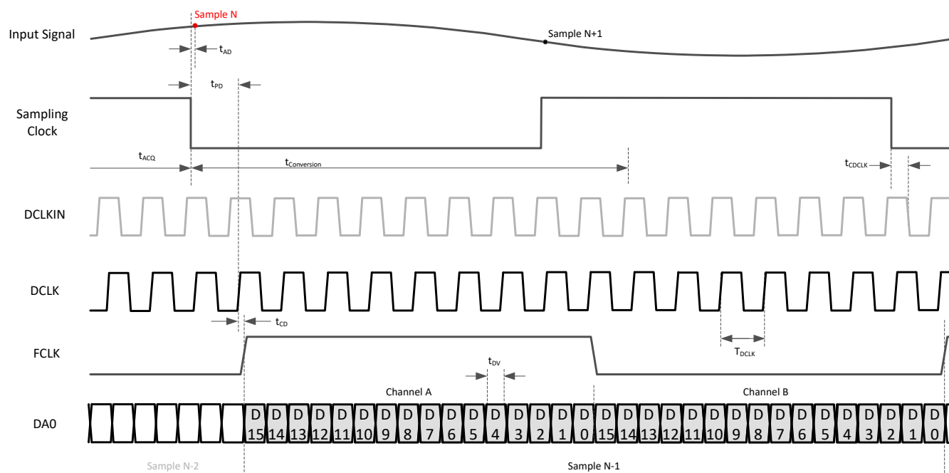
图 7-3. Timing diagram:1/2-wire SLVDS
