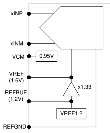
图 8-15. Different voltage reference options for ADC366x
