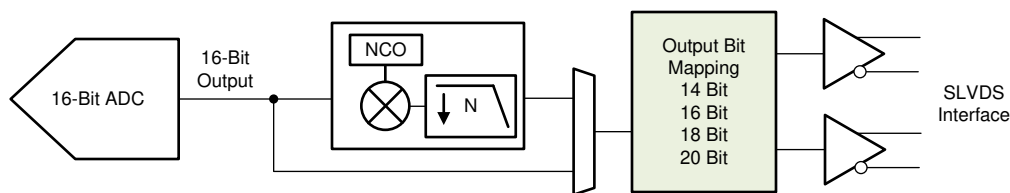
图 8-38. Interface output bit mapper
